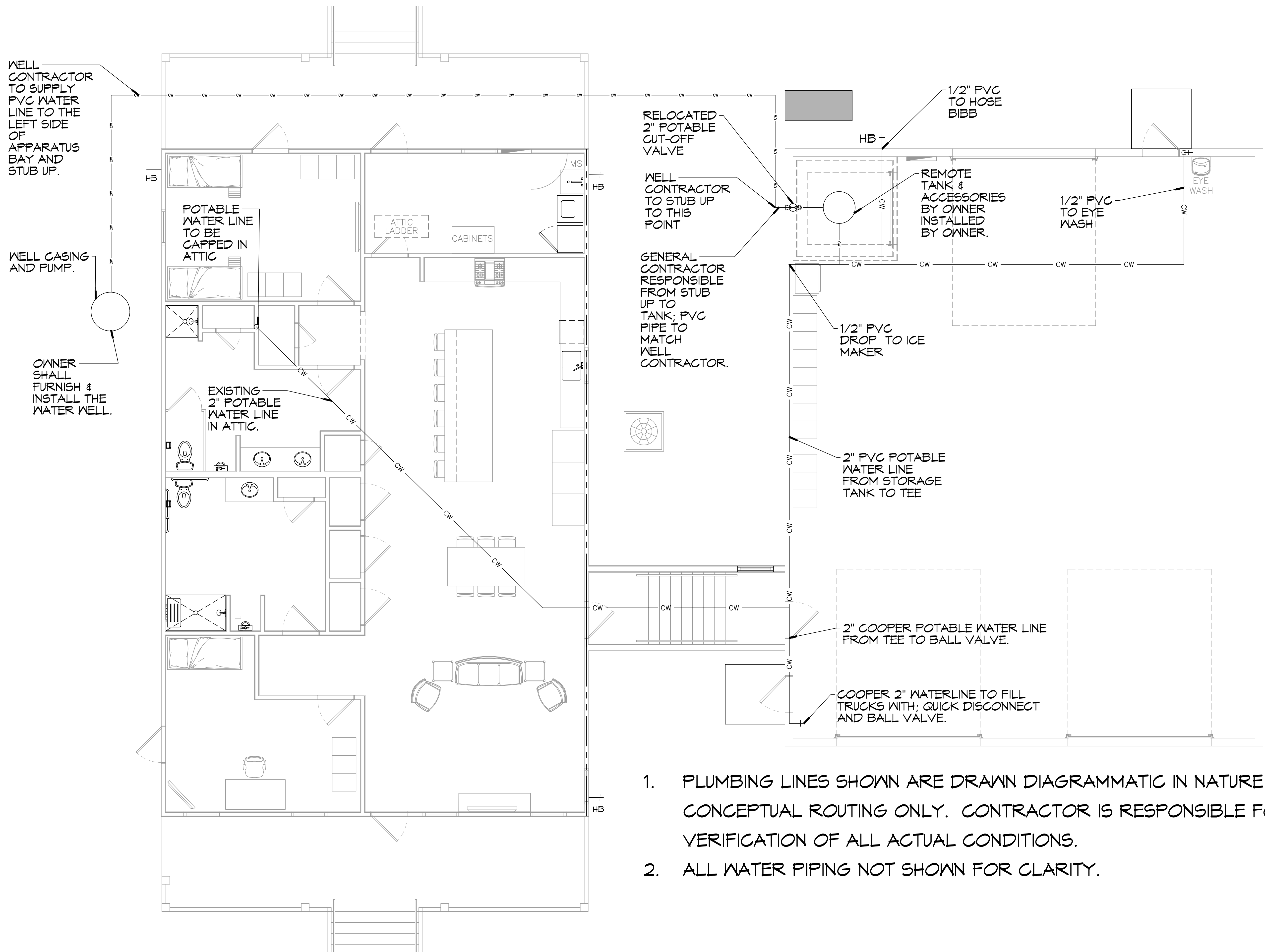
1 WATER WELL AND WATER MAIN(S) PLAN SCALE: 1/4" = 1'-0"
