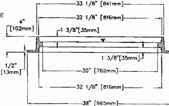
REVERSIBLE RING SECTION
