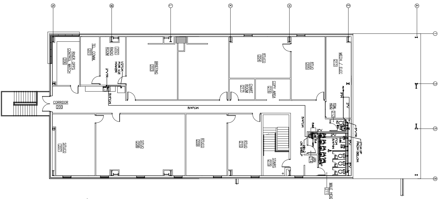
OPERATIONS BUILDING SECOND FLOOR PLUMBING PLAN SCALE: 3/32"=1'-0"
