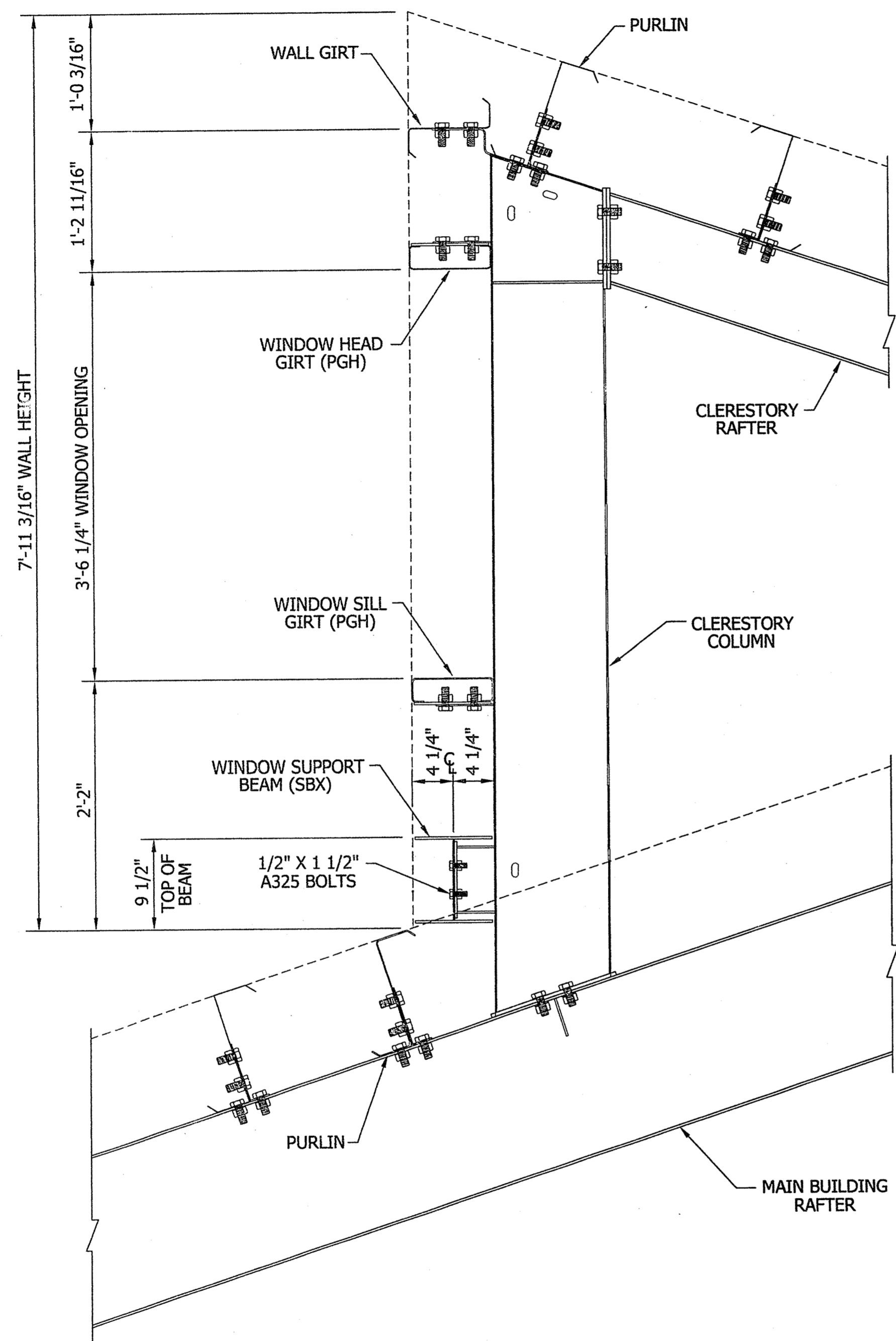
SECTION "3"
