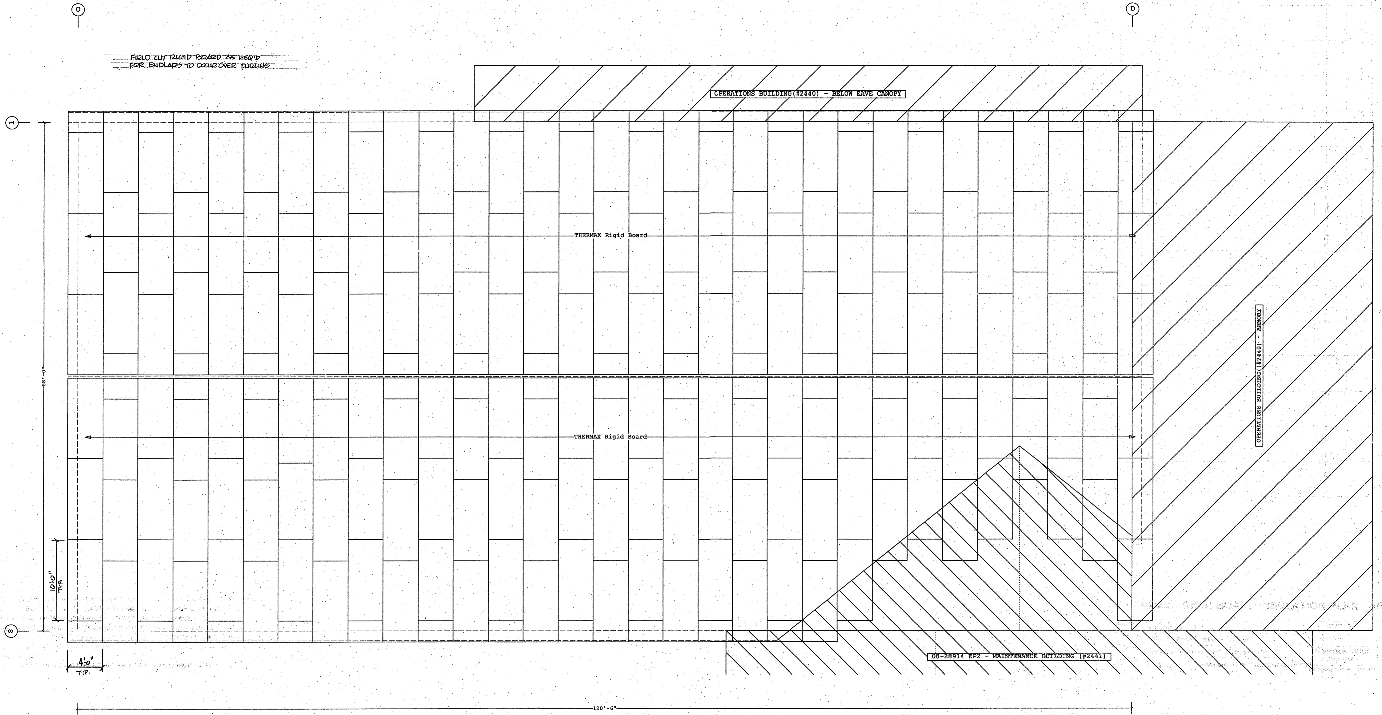
THERMAX - RIGID BOARD INSULATION PLAN - MAIN BLDG.
