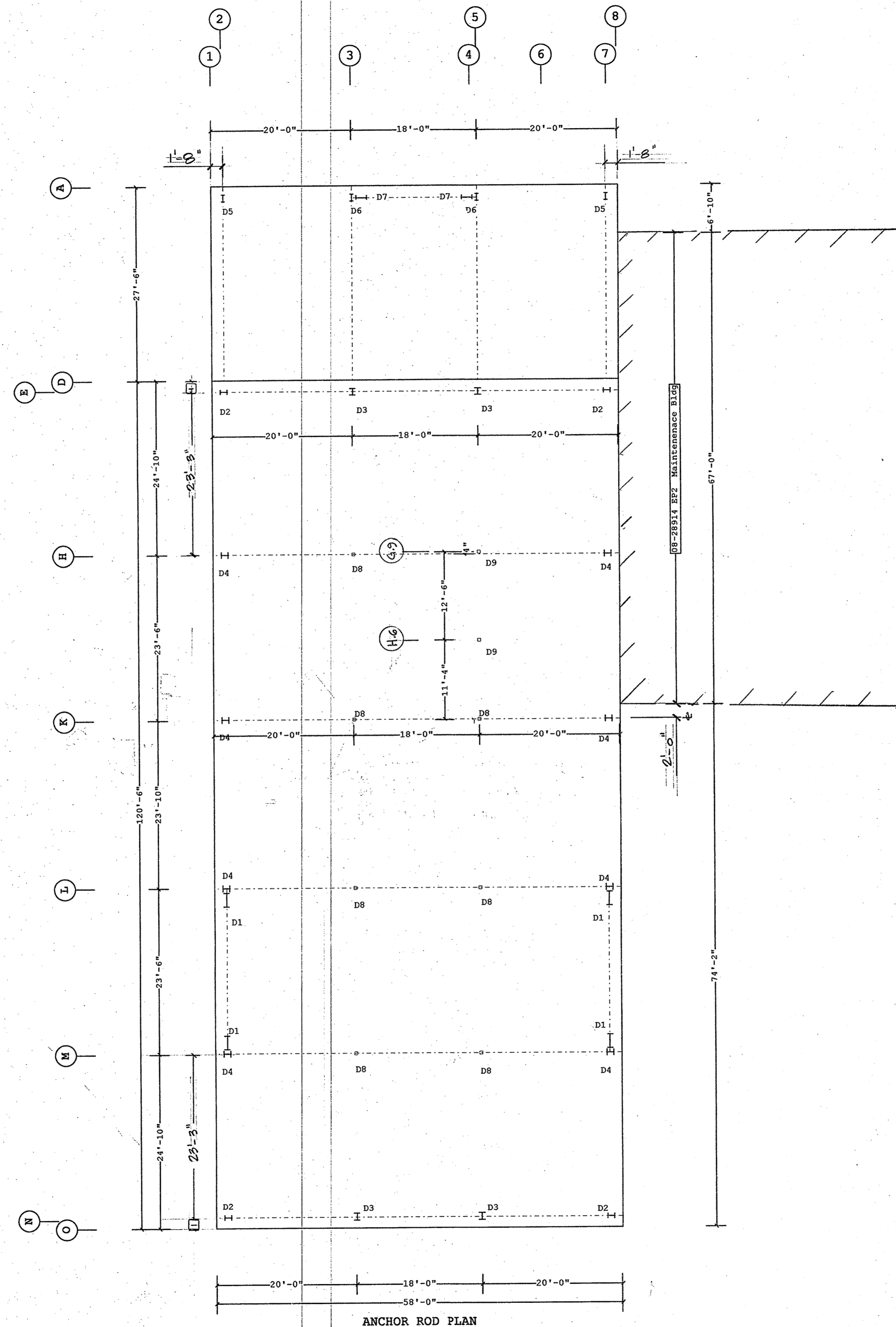
ANCHOR ROD PLAN
