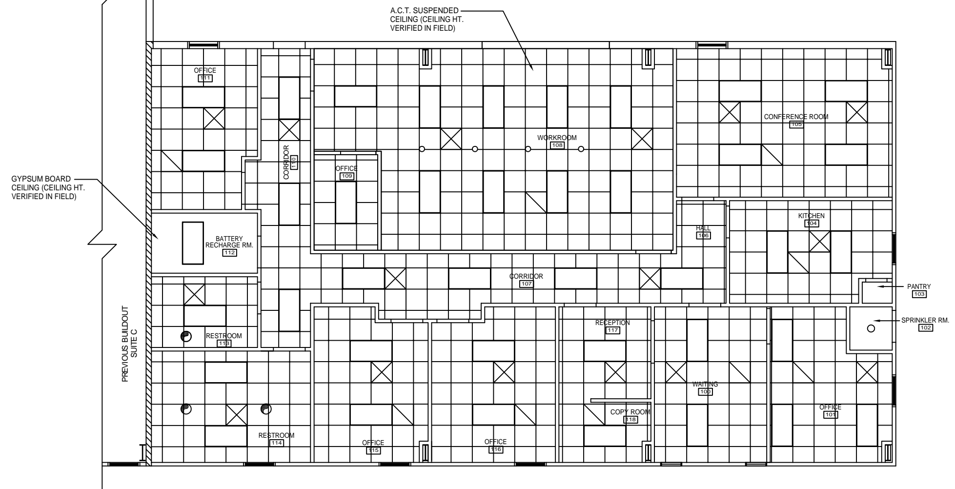
REFLECTED CEILING PLAN - SUITE D SCALE: 1/4"=1'
