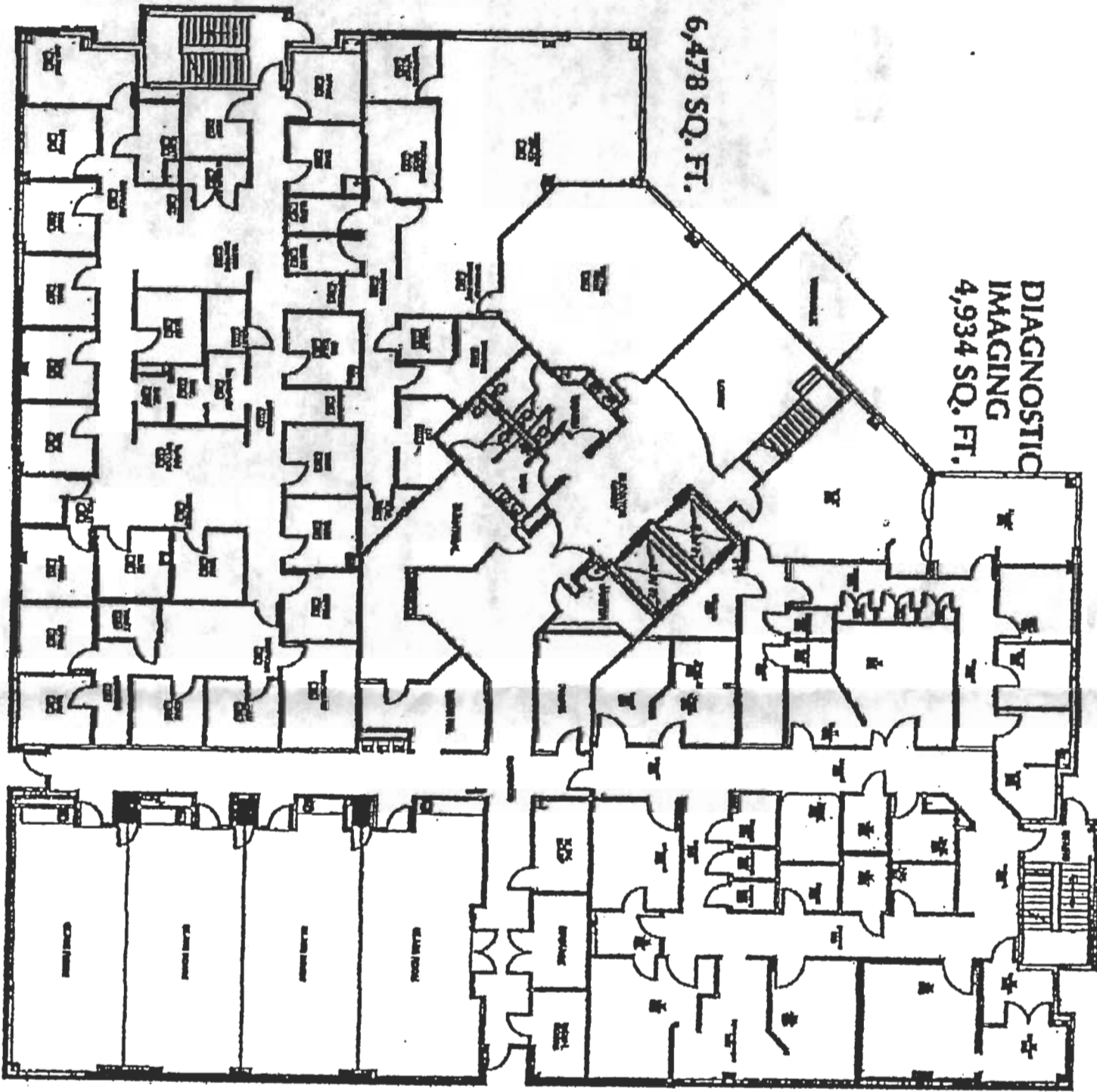
1st Floor Plan - With Tenant Suites July, 2000
