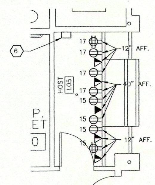
2 FRONT DESK PARTIAL PLAN E-B SCALE: 1/4"=1'-0"
