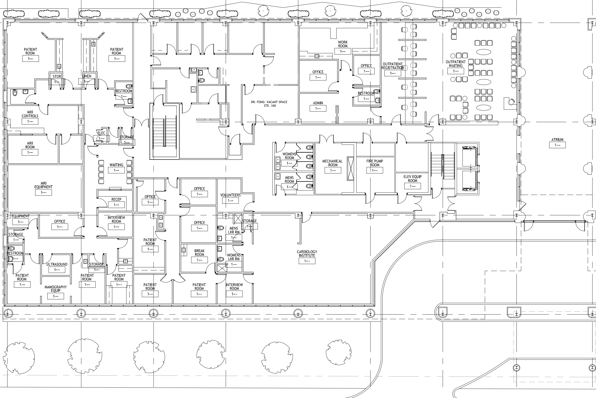
1 EXISTING FLOOR PLAN NTS
