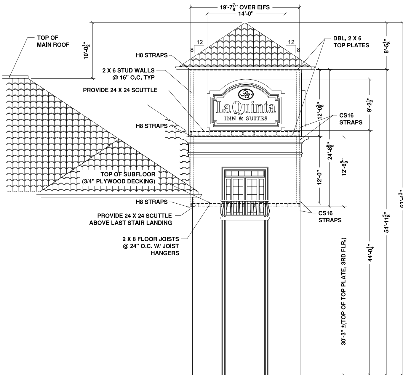
EAST ELEVATION
