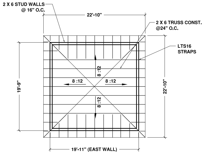
TOWER ROOF FRAMING PLAN
