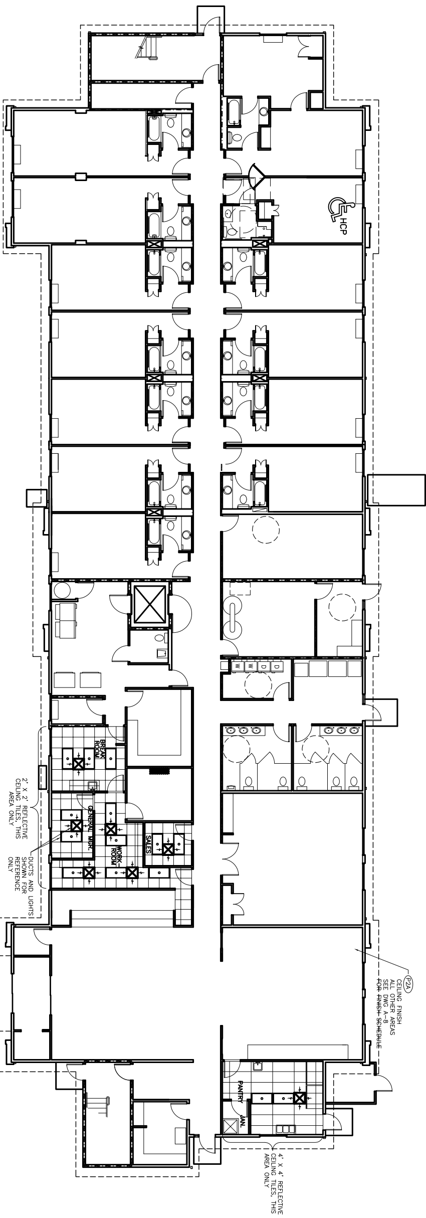
FIRST FLOOR REFLECTIVE CEILING PLAN SCALE: 1/8"=1'-0"
