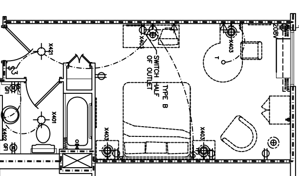
ELECTRICAL PLAN UNIT TYPE D SCALE: 1/4"=1'-0"
