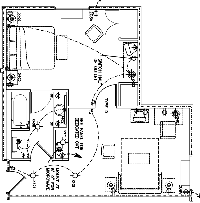
ELECTRICAL PLAN UNIT TYPE "E" SCALE: 1/4"=1'-0"
