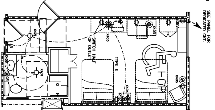
ELECTRICAL PLAN UNIT TYPE "F" SCALE: 1/4"=1'-0"
