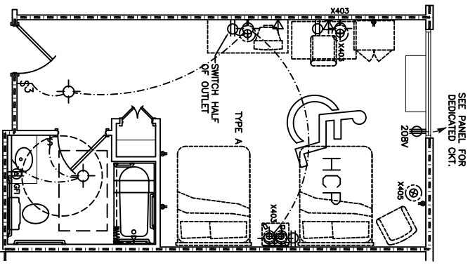
ELECTRICAL PLAN UNIT TYPE A SCALE: 1/4"=1'-0"
