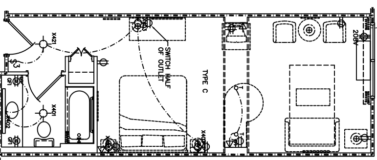
ELECTRICAL PLAN UNIT TYPE C SCALE: 1/4"=1'-0"
