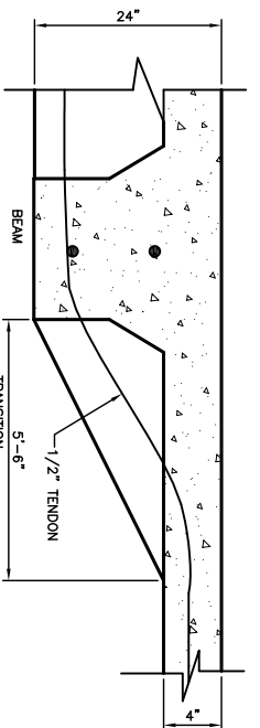
TYPICAL BEAM ENDS INTO SLAB N.T.S.
