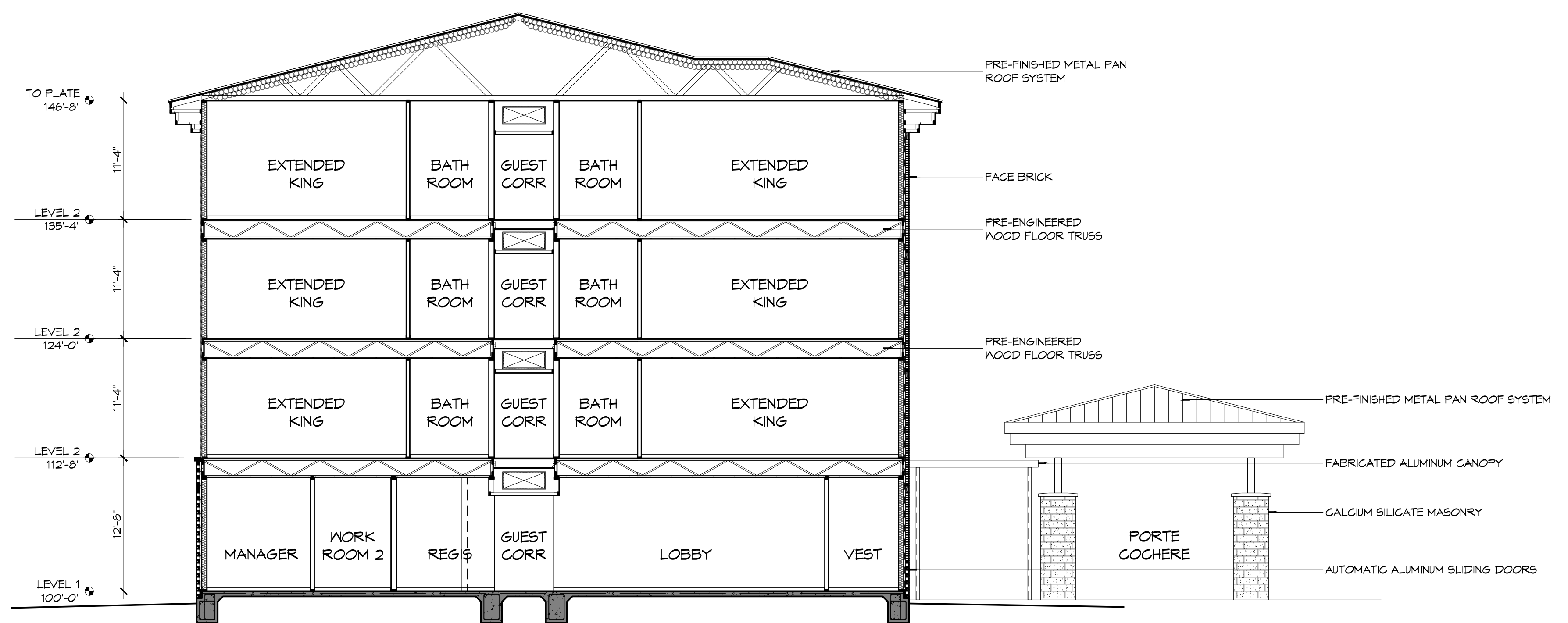
1 BUILDING SECTION SCALE: 1/8" = 1'-0"
