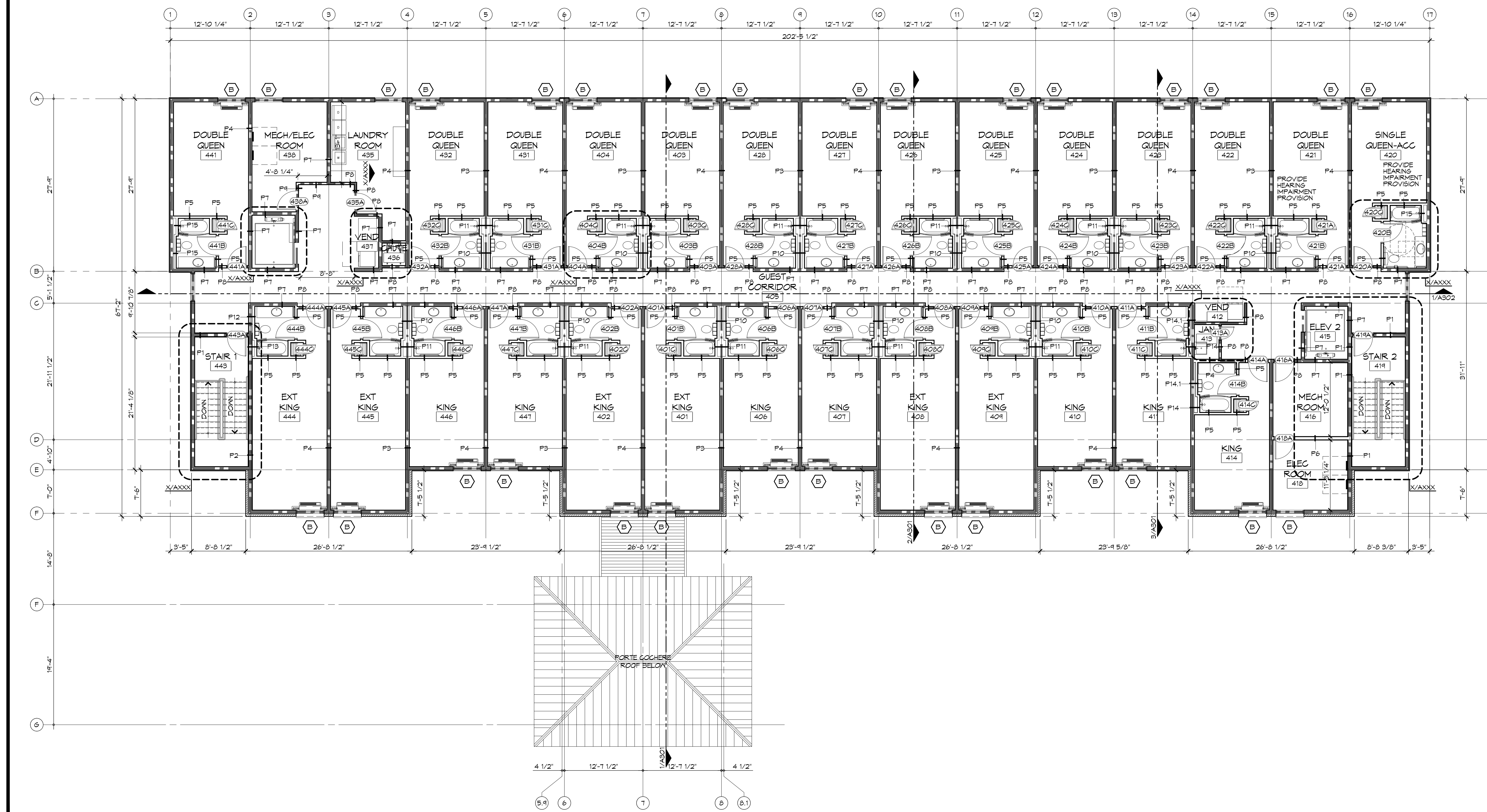
1 ARCHITECTURAL FLOOR PLAN - LEVEL 4 SCALE: 1/8" = 1'-0"
