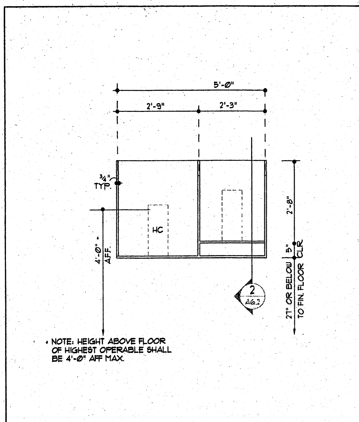
1 Section Detail Phone Elevation SCALE: 1/2" = 1'-0"
