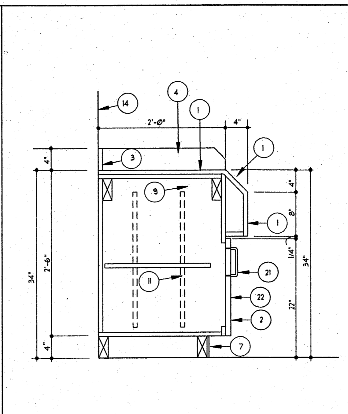
3 Section Detail Breakfast Bar Counter SCALE: 1" = 1'-0"
