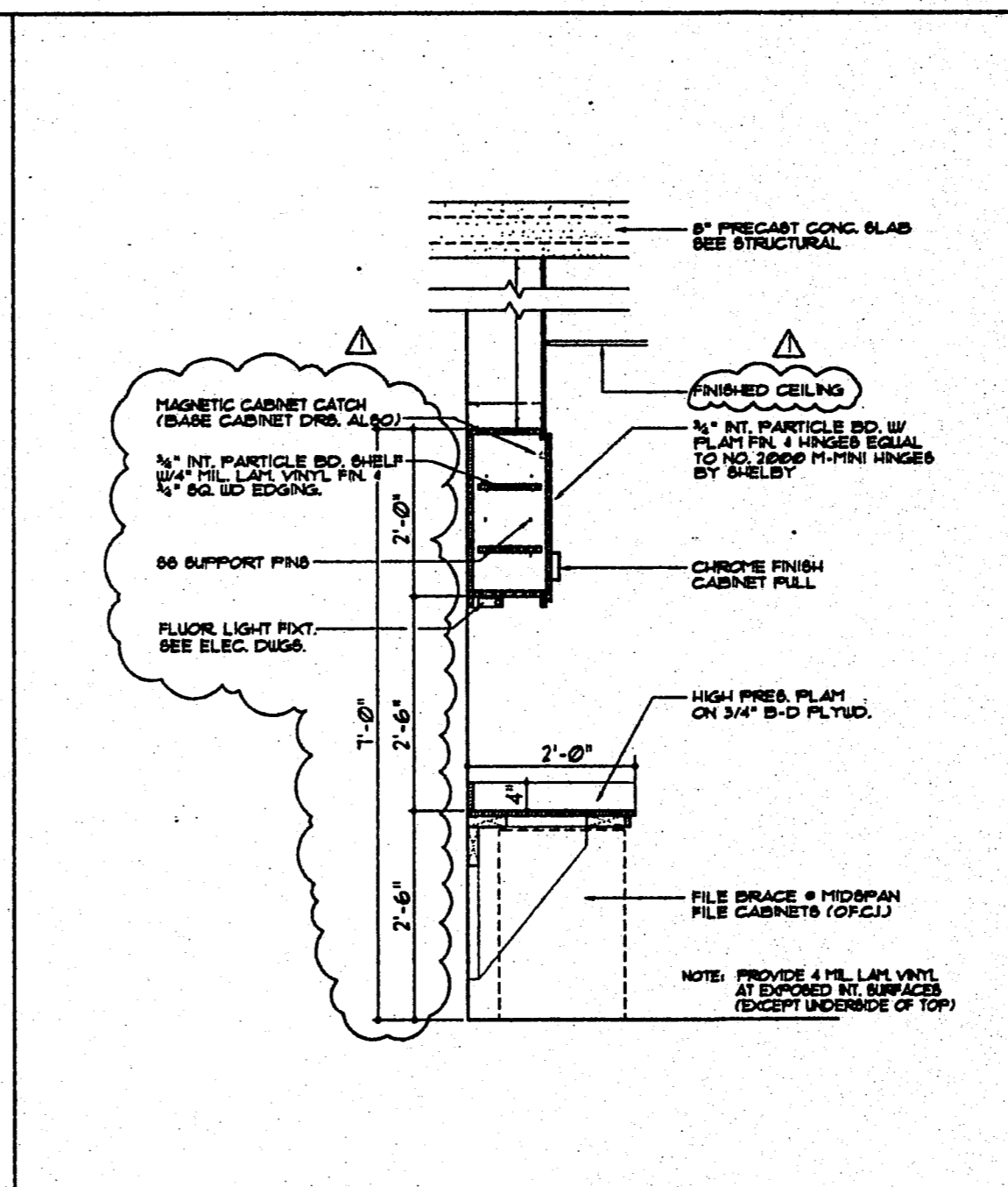
4 Section Detail Work Area SCALE: 1/2" = 1'-0"
