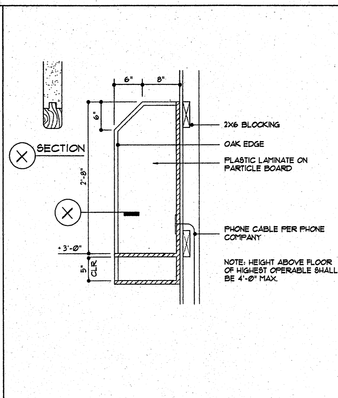
2 Section Detail Phone Shelf SCALE: 1" = 1'-0"
