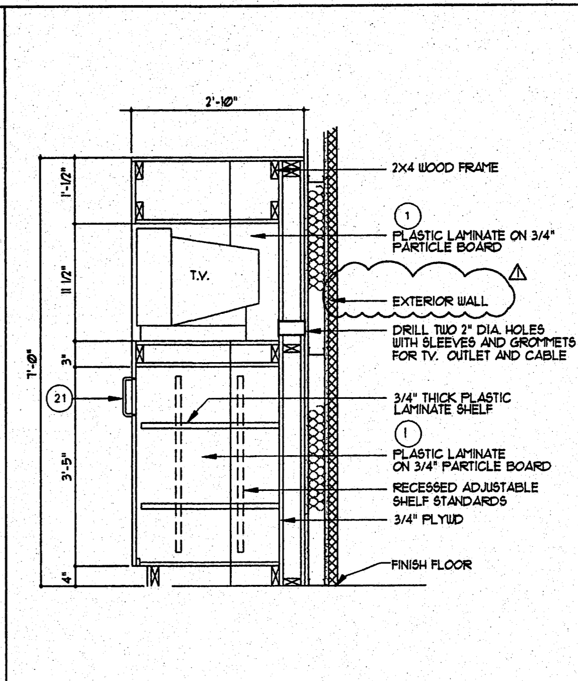
5 Section Detail TV Unit SCALE: 3/4" = 1'-0"
