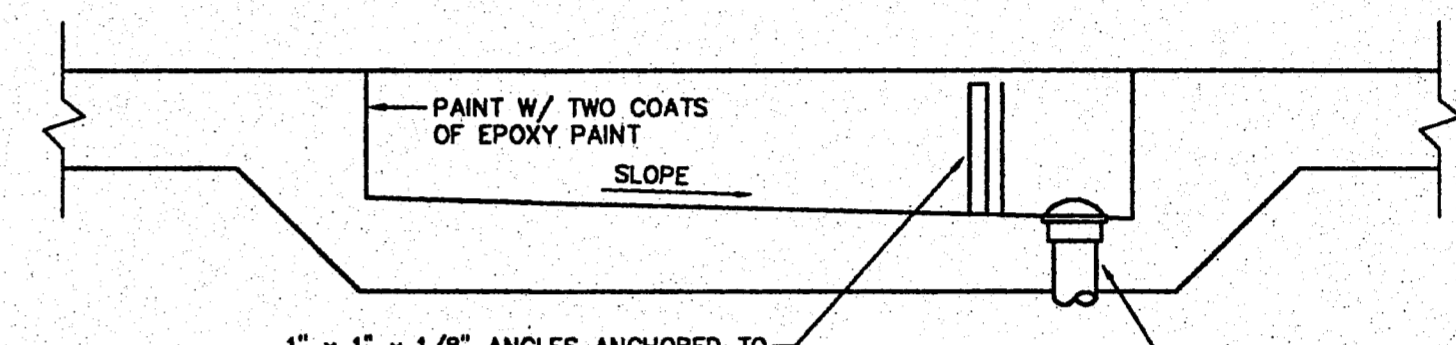
WASHER TRENCH DETAIL NOT TO SCALE
