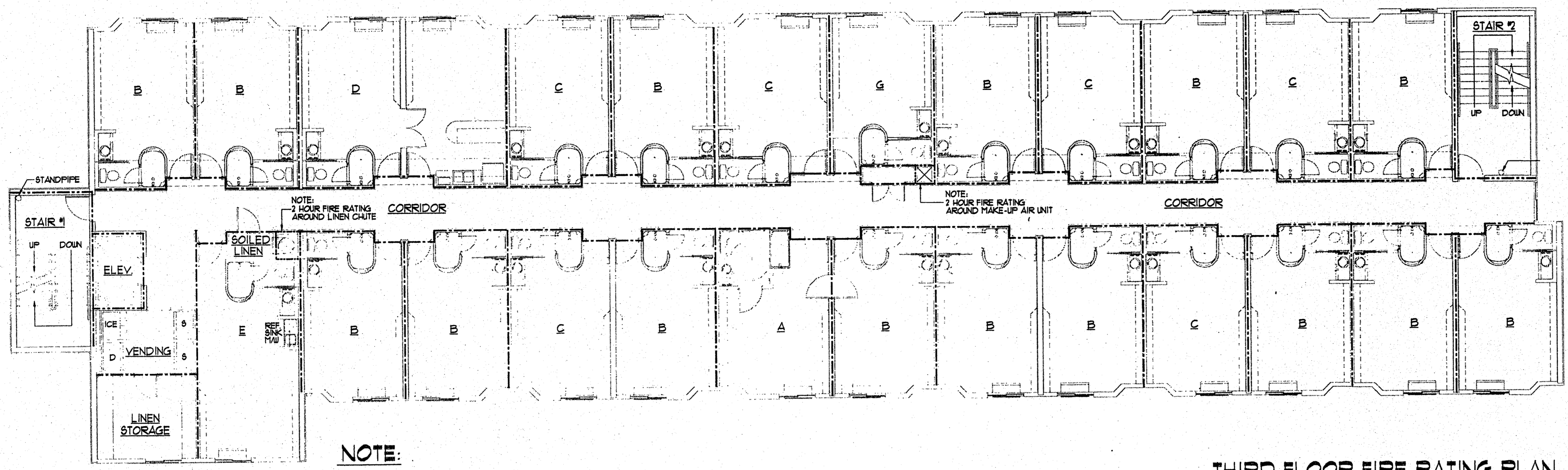
THIRD FLOOR FIRE RATING PLAN SCALE: 1/8" = 1'-0"
