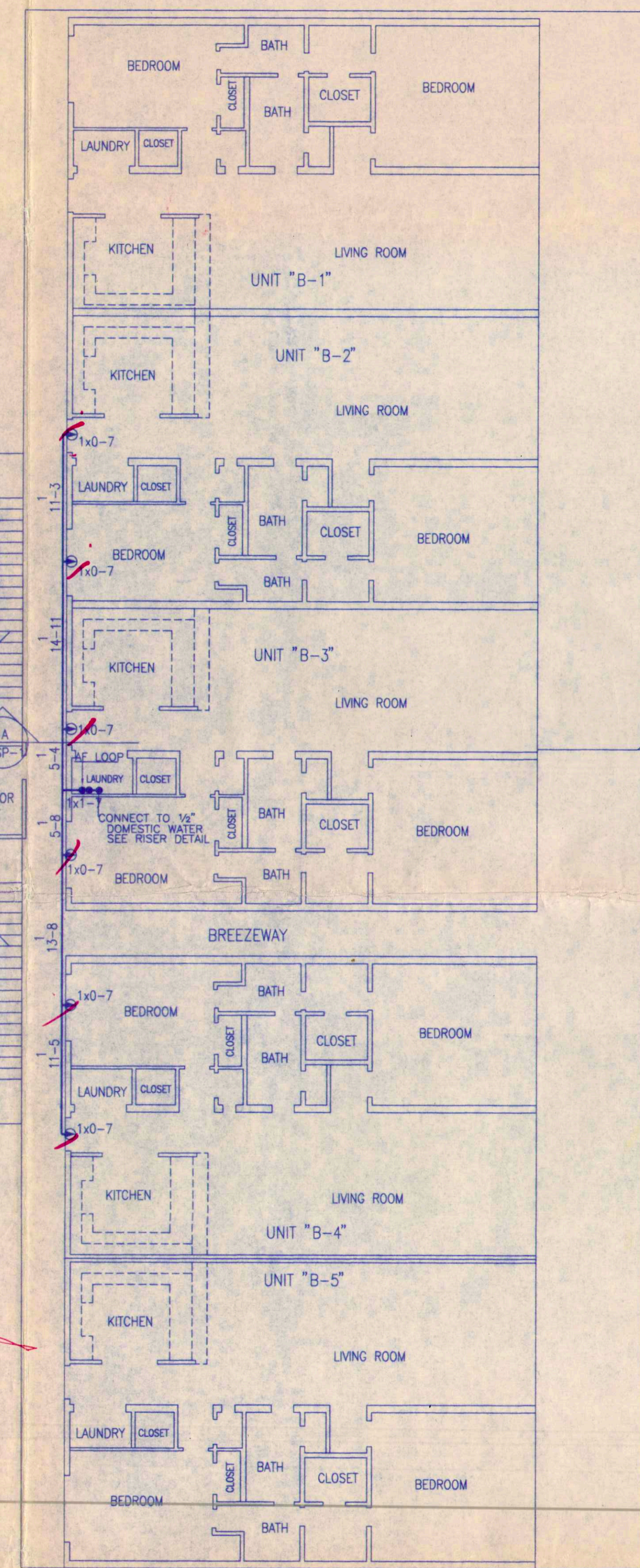
2ND FLOOR SPRINKLER PLAN SCALE: 1/8" = 1'-0"
