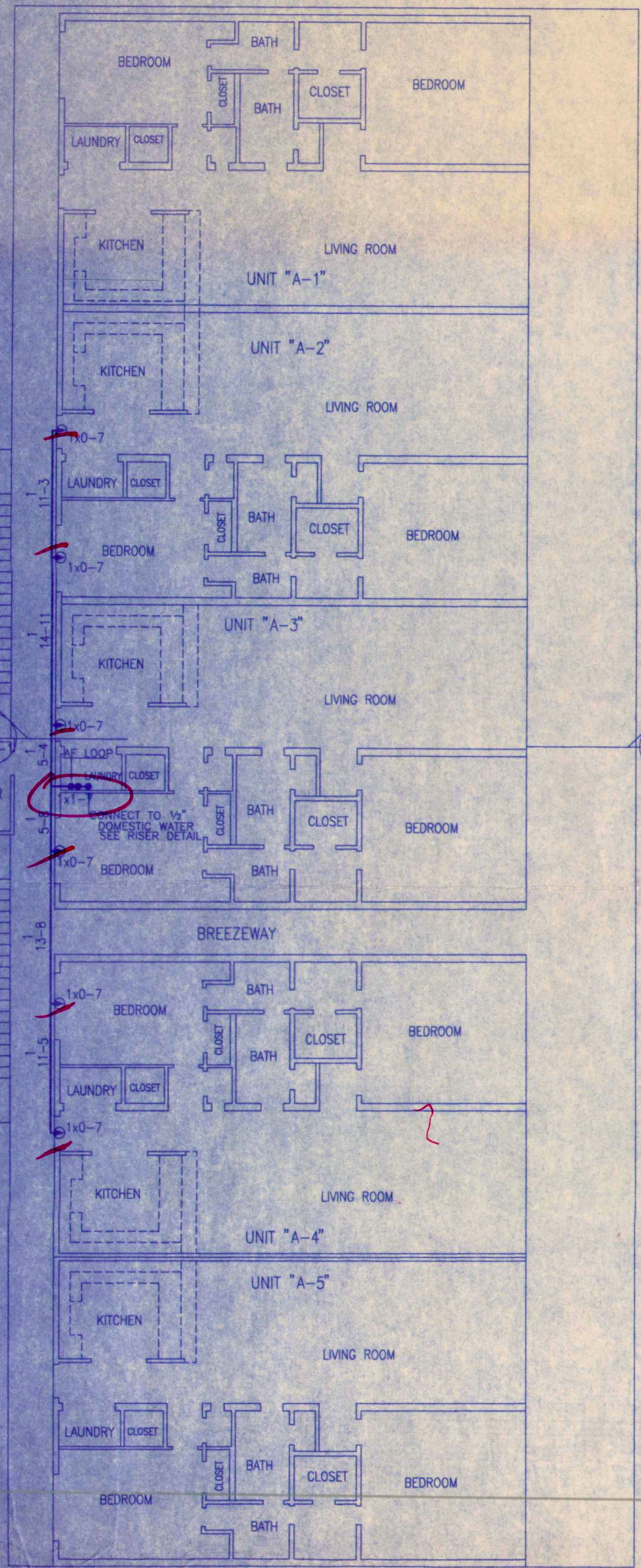
1ST FLOOR SPRINKLER PLAN SCALE: 1/8" = 1'-0"
