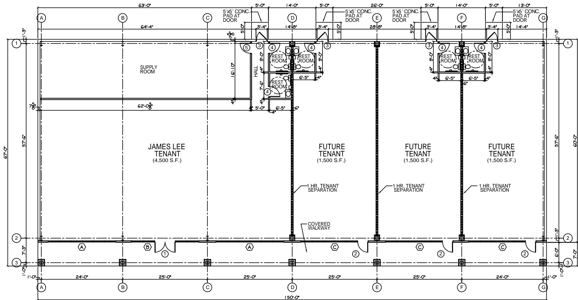
FLOOR PLAN SCALE: 1/8"=1'
