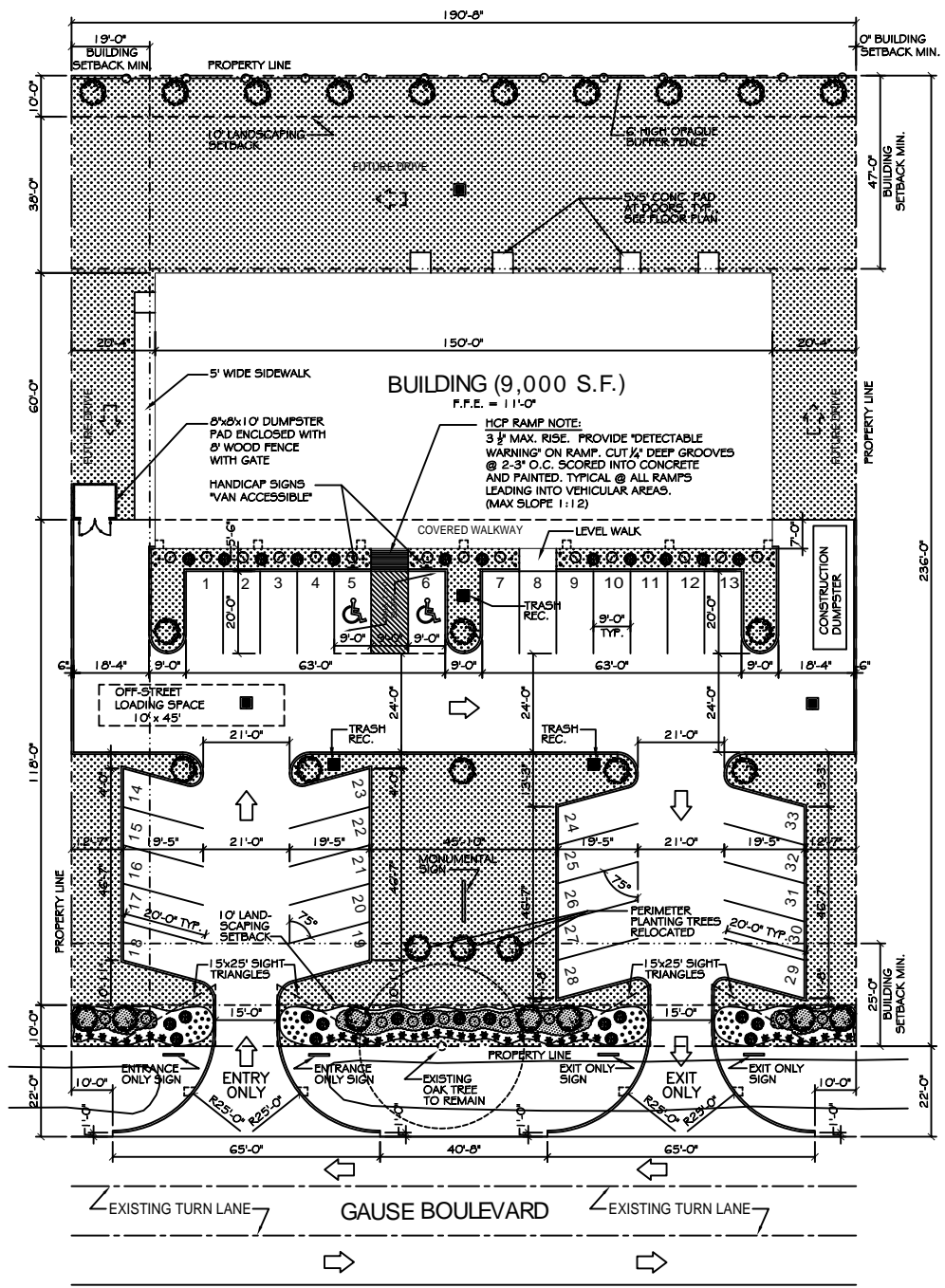
SITE PLAN SCALE: 1"=20'
