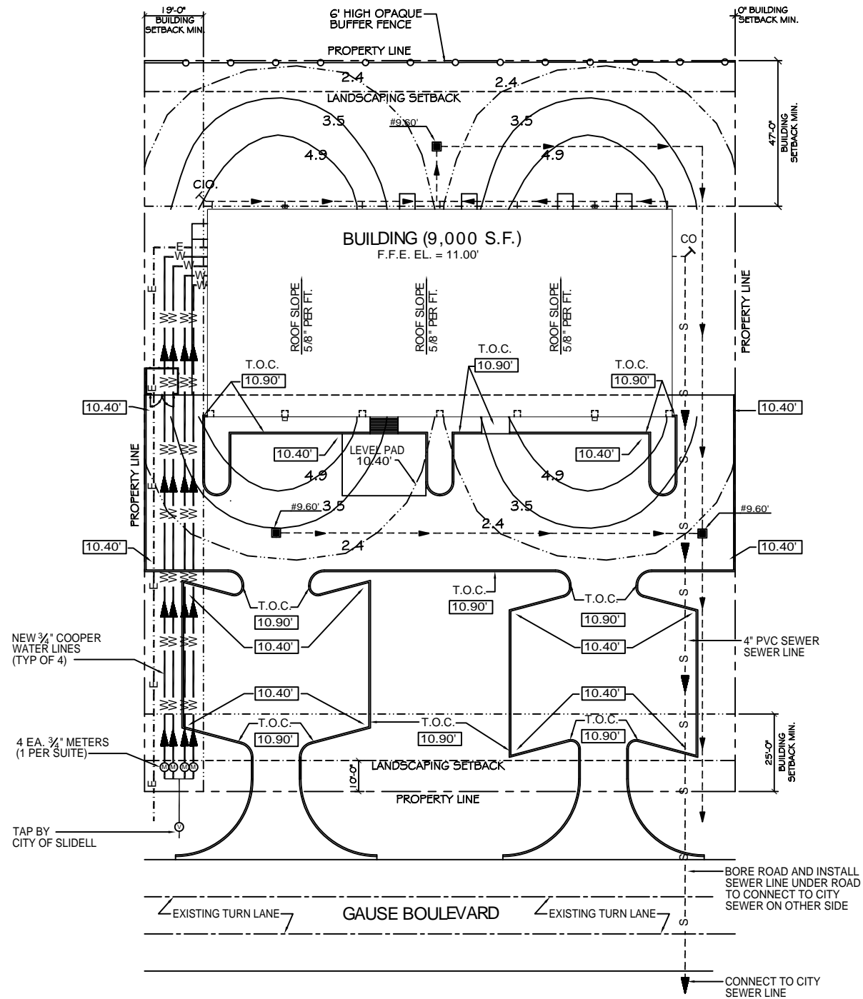
SITE UTILITIES & ILLUMINATION PLAN SCALE: 1"=20'
