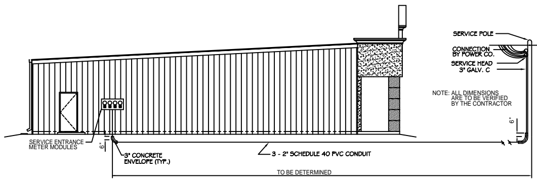
ELECTRICAL SERVICE DETAIL N.T.S.
