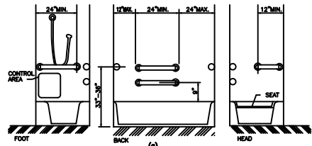
FIG. 32 GRAB BARS AT BATHTUBS N.T.S.
