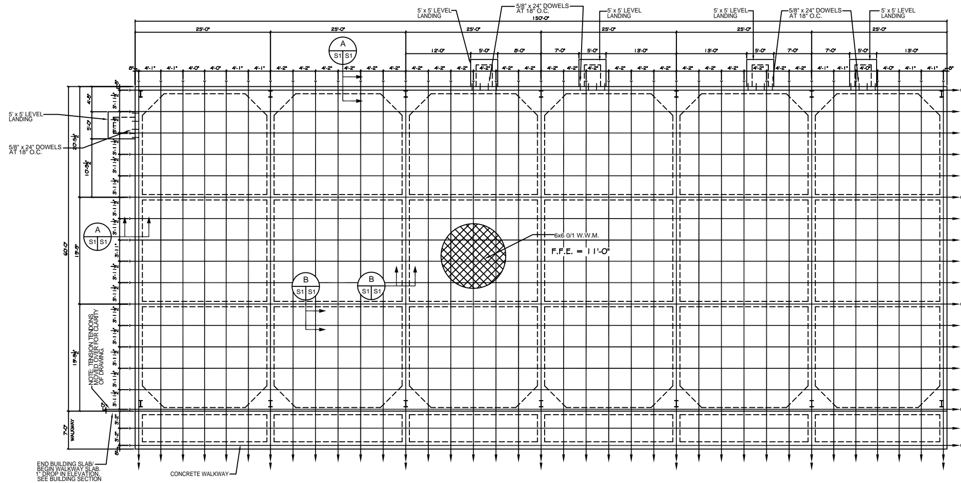
FOUNDATION PLAN SCALE: 1/8"=1'
