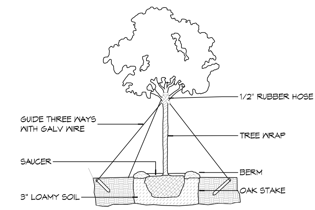
C TYPICAL TREE PLANTING
