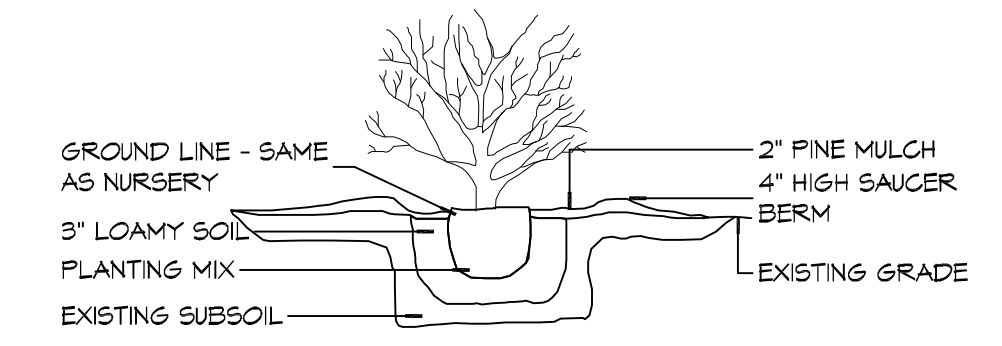
B TYPICAL SHRUB PLANTING
