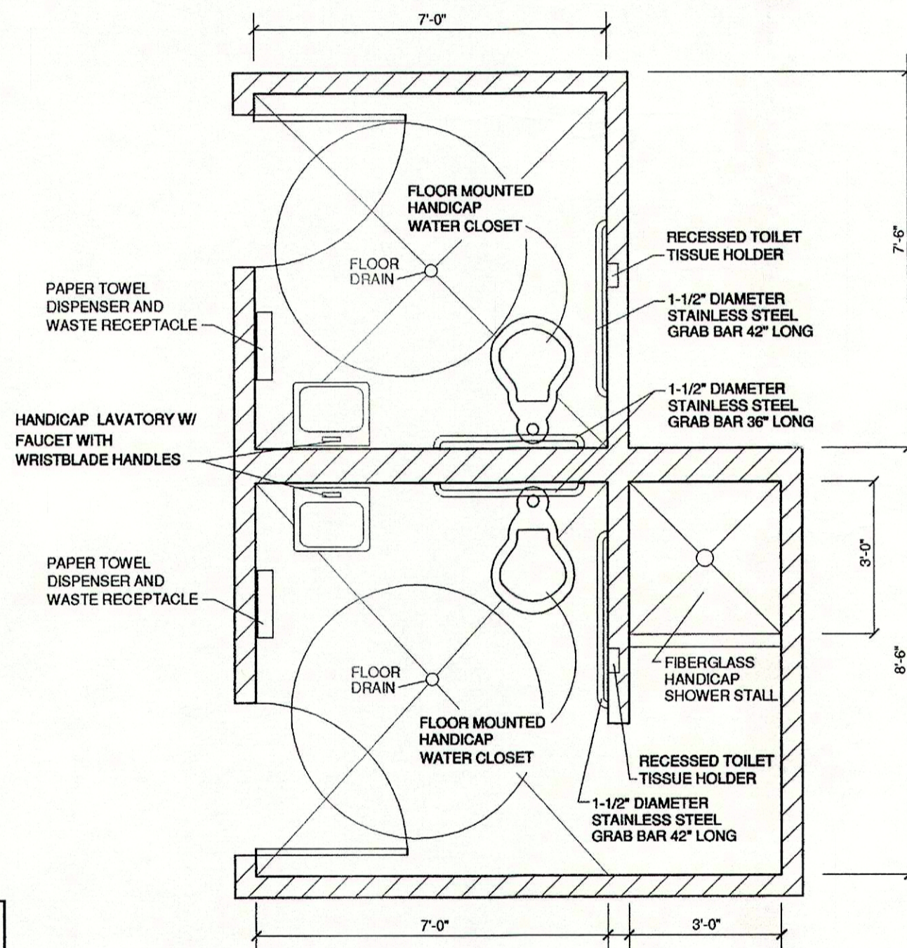
3 PLAN (TYP.) A7 SCALE 3/8" = 1'-0"
