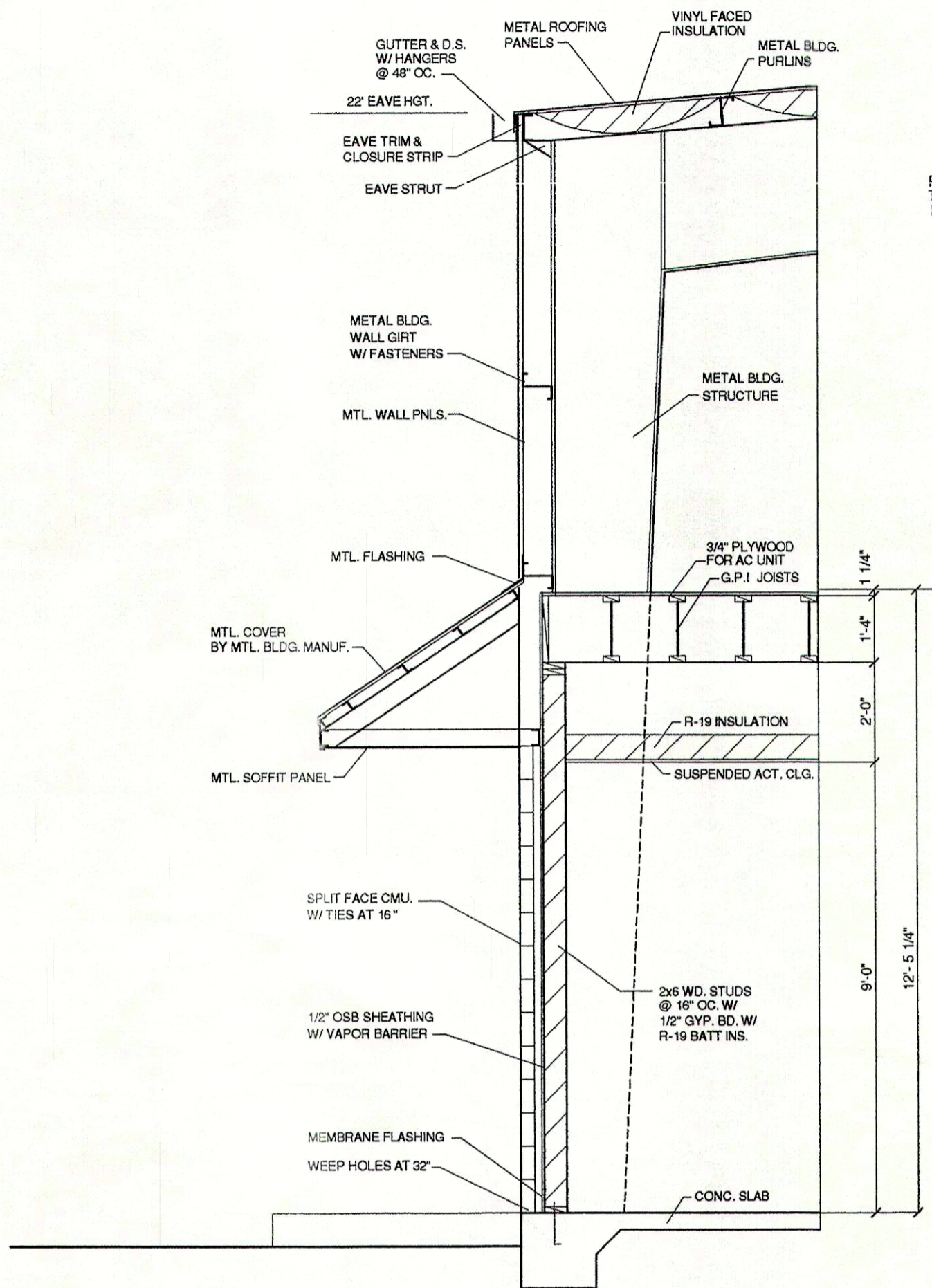
4 WALL SECTION A7 SCALE 3/8" = 1'-0"
