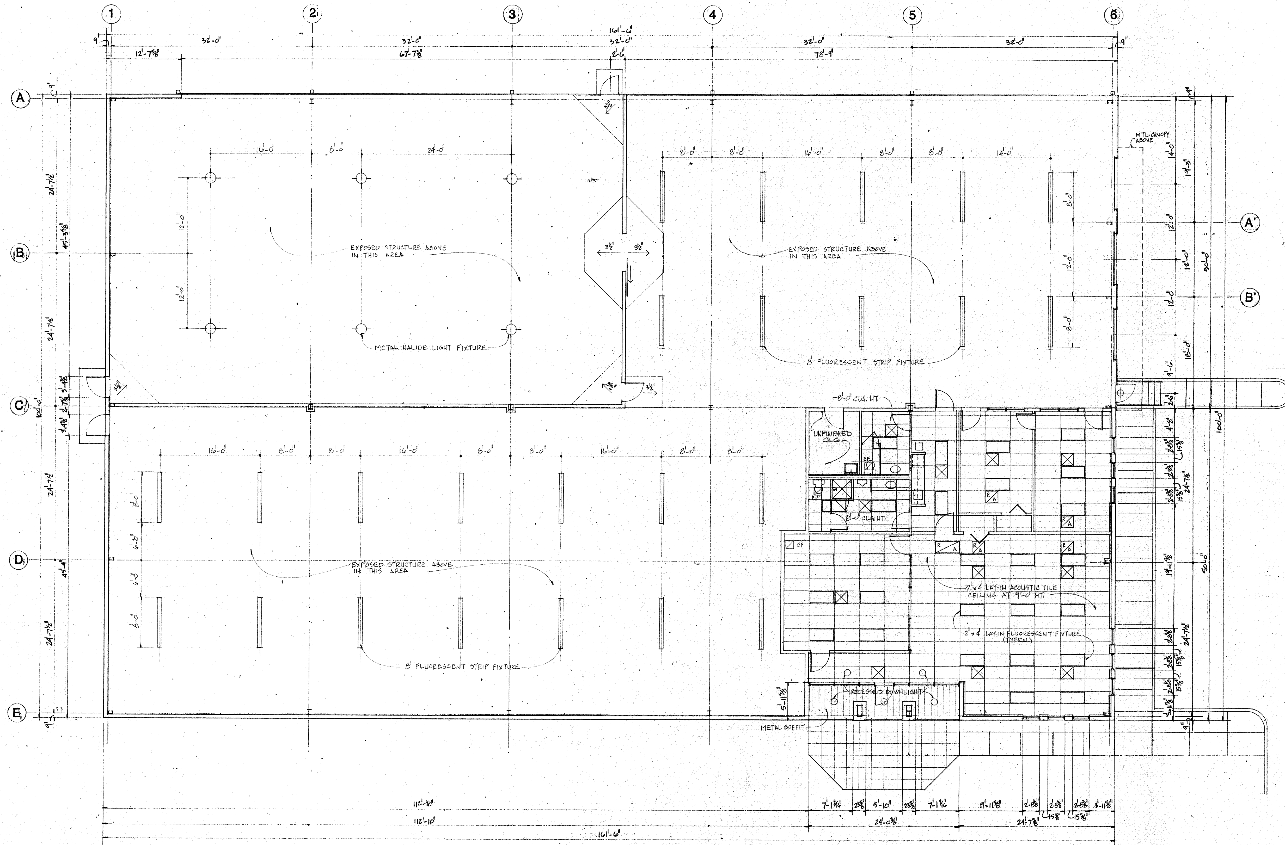
reflected ceiling plan scale: 1/8"=1'-0"
