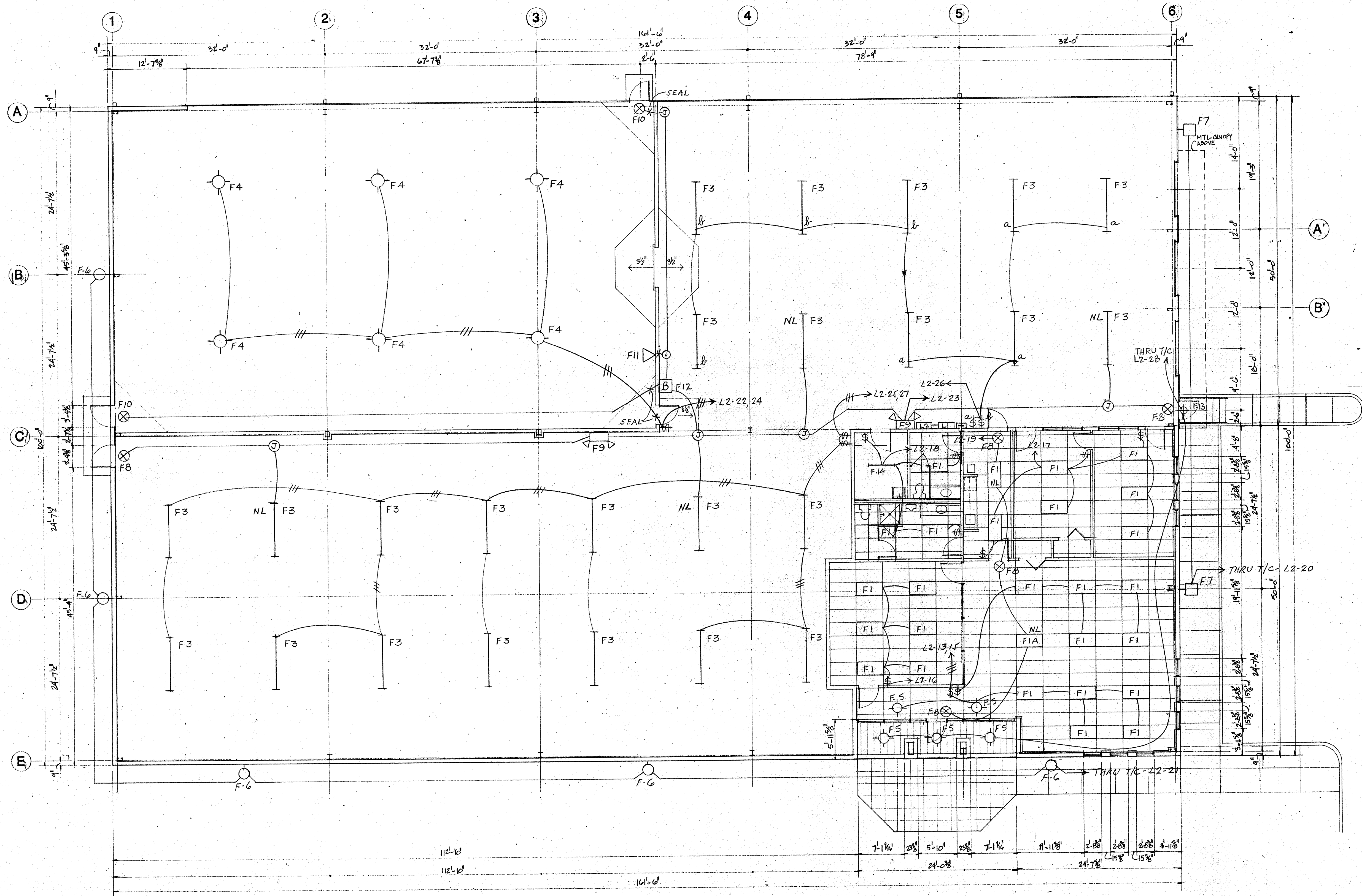
lighting plan scale: 1/8"=1'-0"
