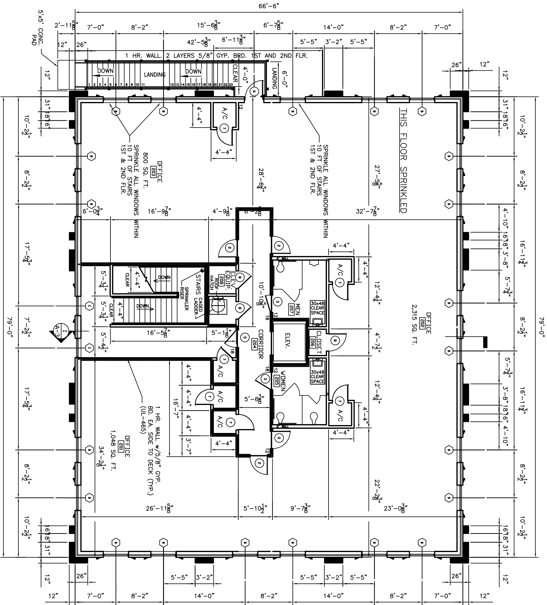
FRONT OF BUILDING SECOND FLOOR PLAN SCALE: 3/16"=1'-0"
