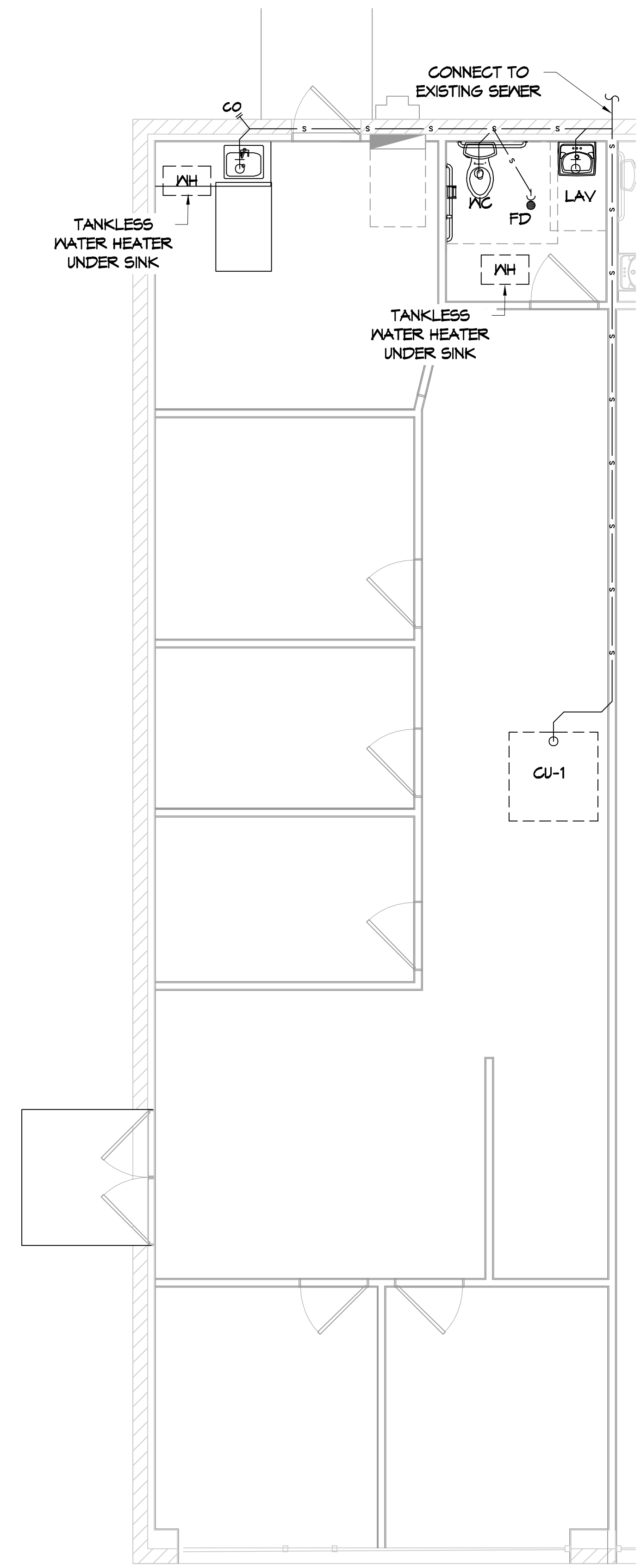
10 PLUMBING PLAN SCALE: 1/4"=1'-0"
