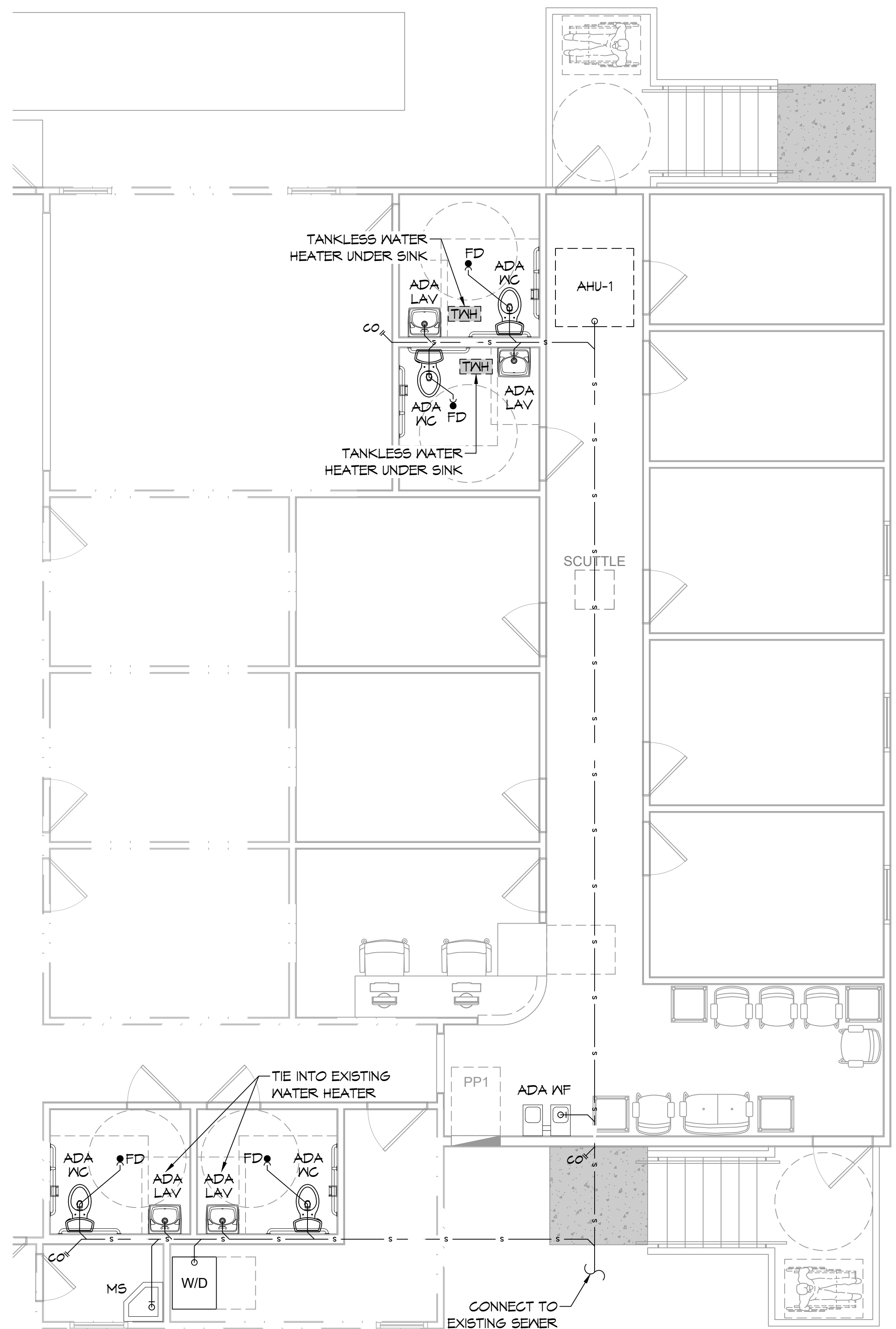
16 PLUMBING PLAN SCALE: 1/4" = 1'-0"
