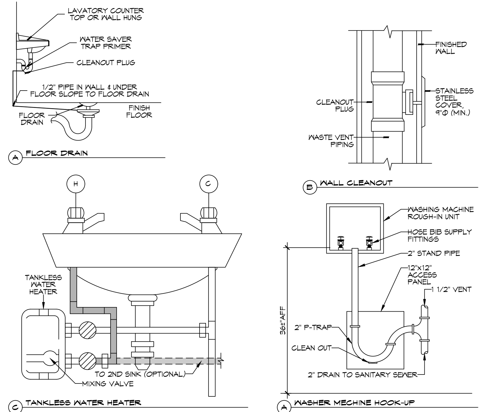
PLUMBING DETAILS SCALE: NTS
