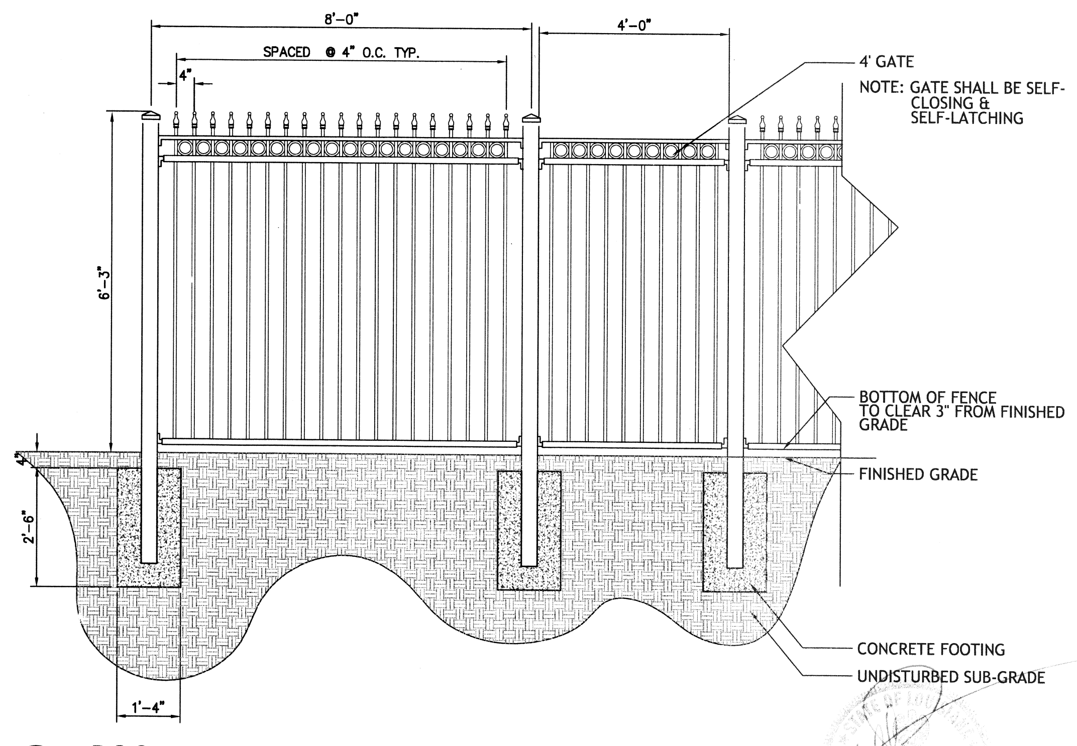
3 POOL ENTRY DETAIL SCALE: 1/2" = 1'-0"
