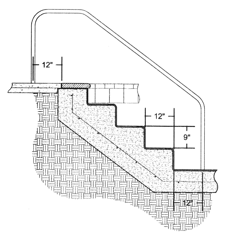
4 POOL ENTRY DETAIL SCALE: 1/2" = 1'-0"
