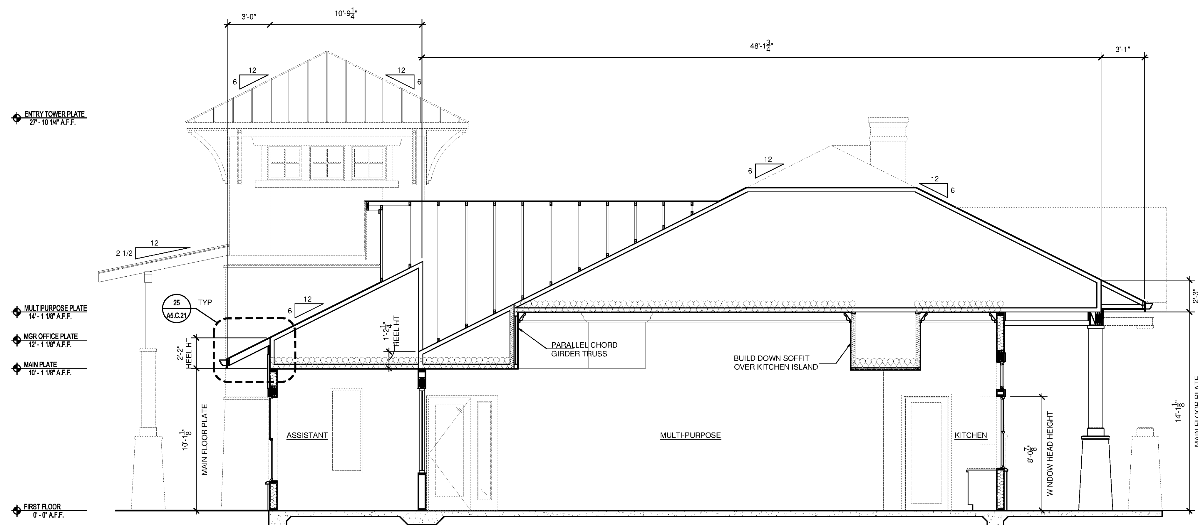
1 BUILDING SECTION - CLUBHOUSE SCALE: 1/4"=1'-0"
