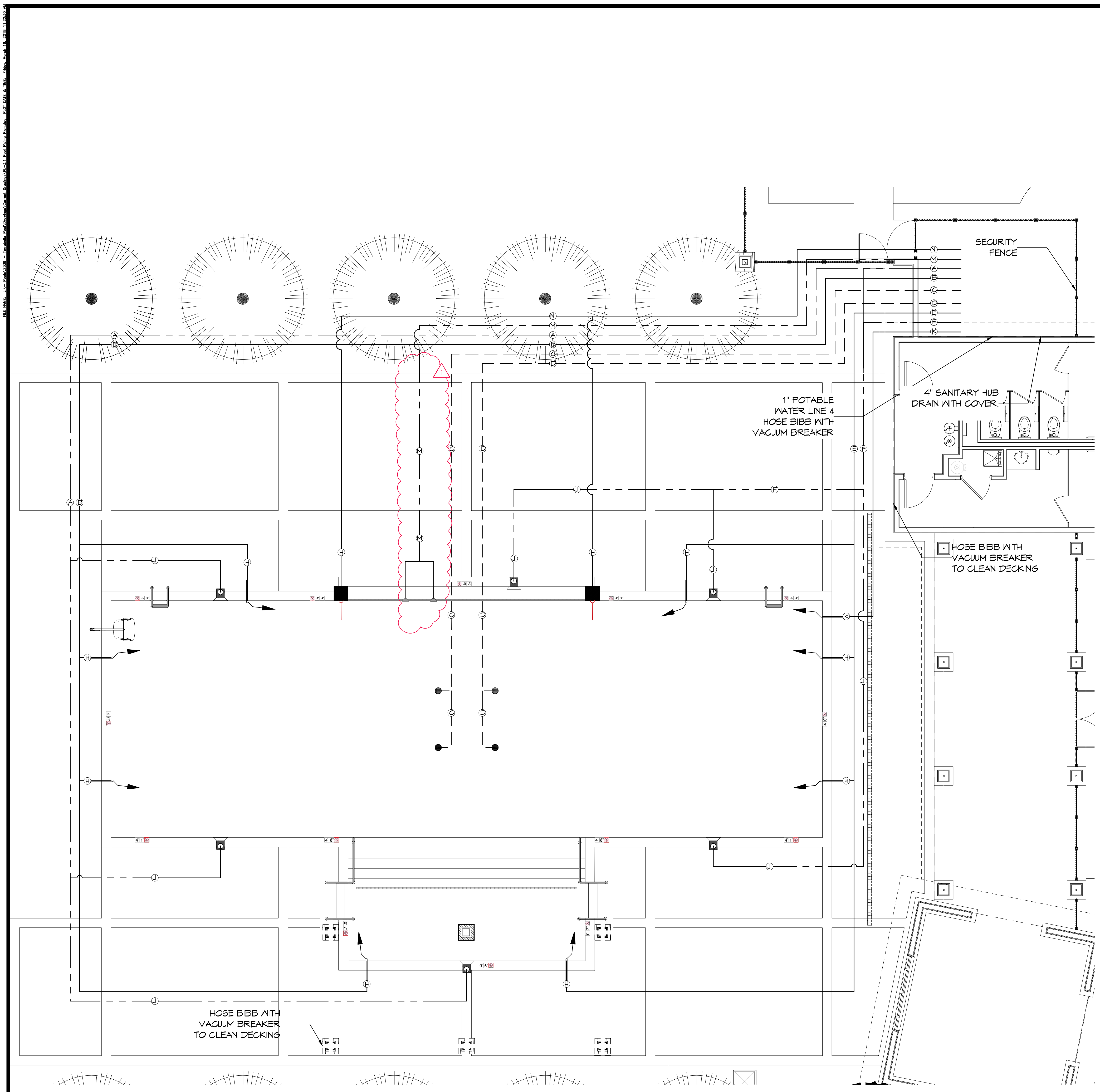
1 POOL PIPING PLAN SCALE: 3/16" = 1'-0"
