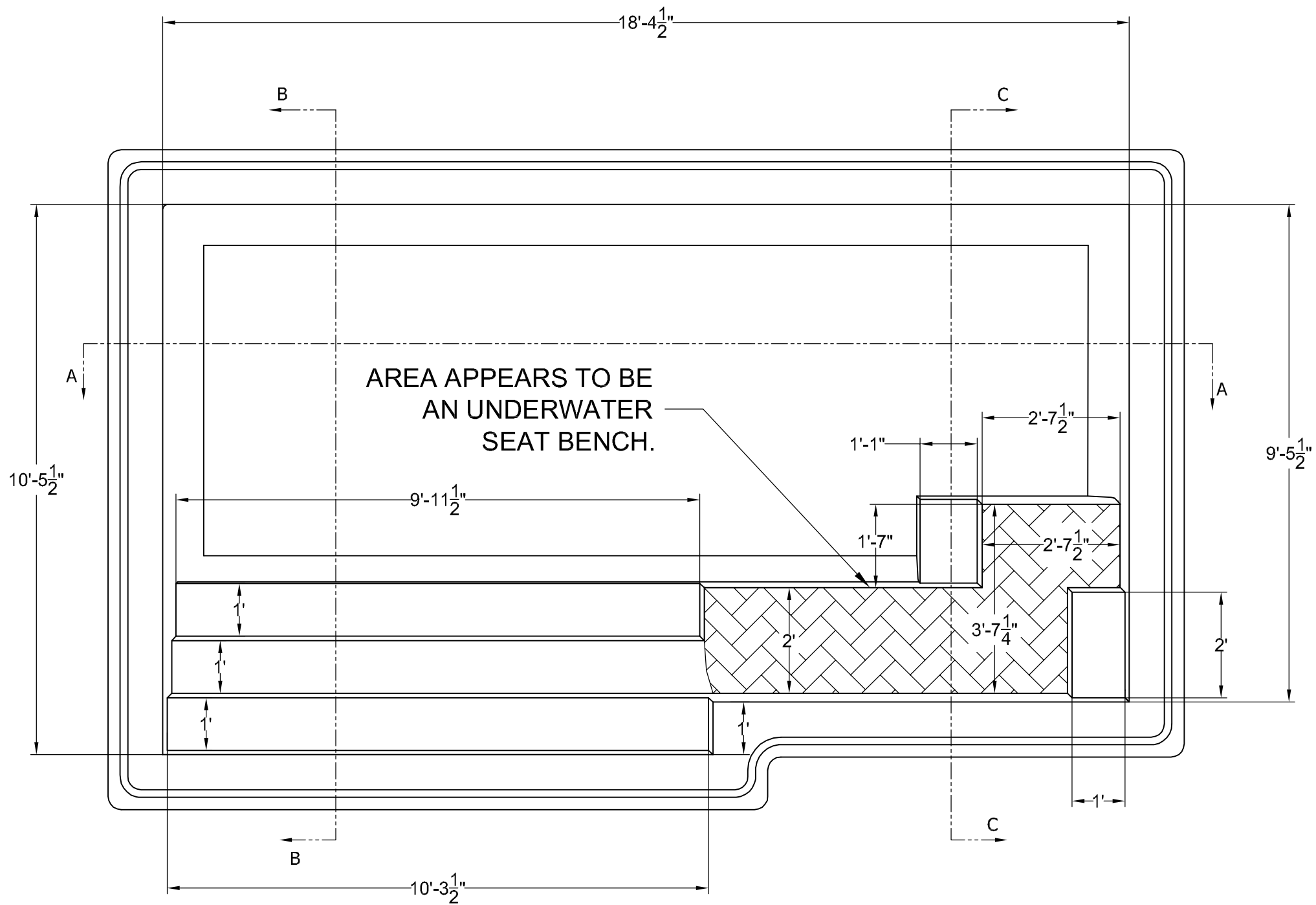
PLAN VIEW
