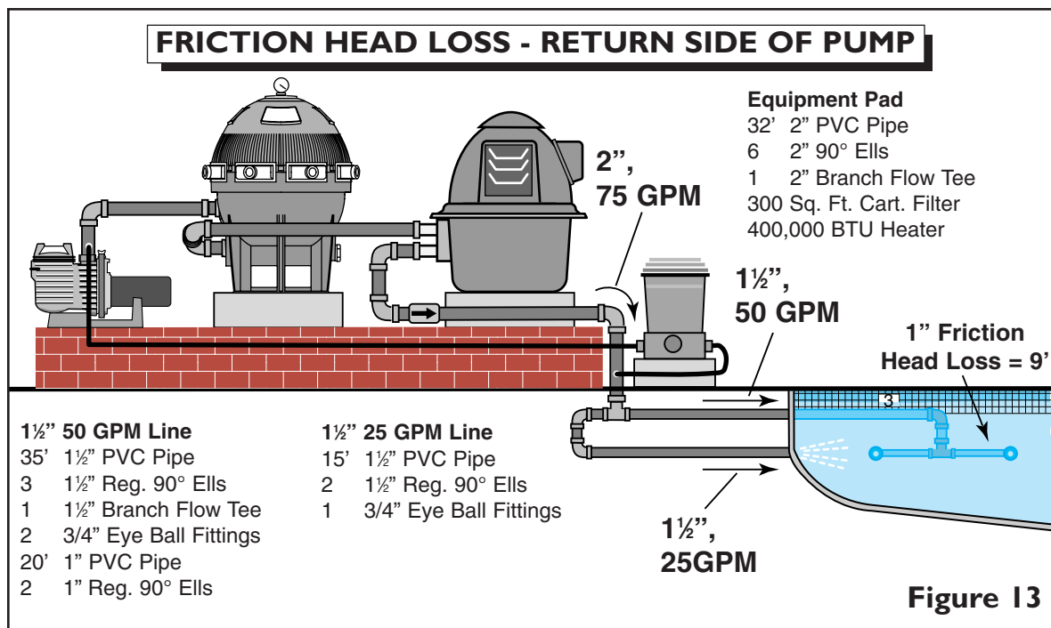
Figure 13 is a typical plumbing layout for multiple return lines. One 2" line Teed into two 1 1/2" lines, one with a single return fitting, the other with two return fittings.
