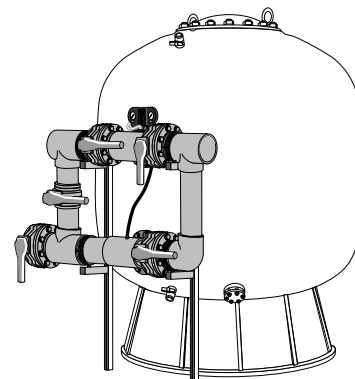
4 - VALVE BACKWASH
