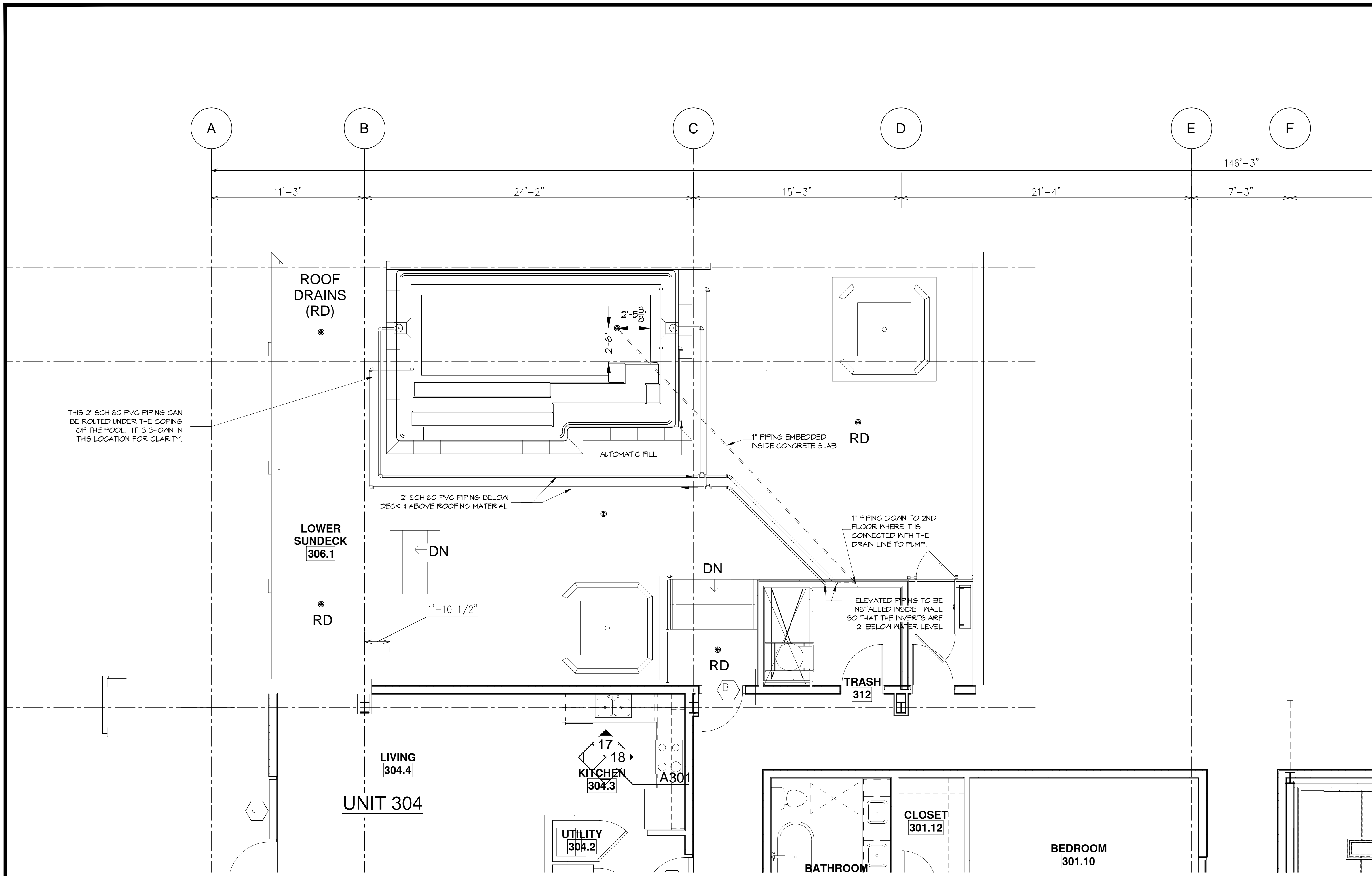
3rd FLOOR POOL PIPING PLAN SCALE: 1/4" = 1'-0"
