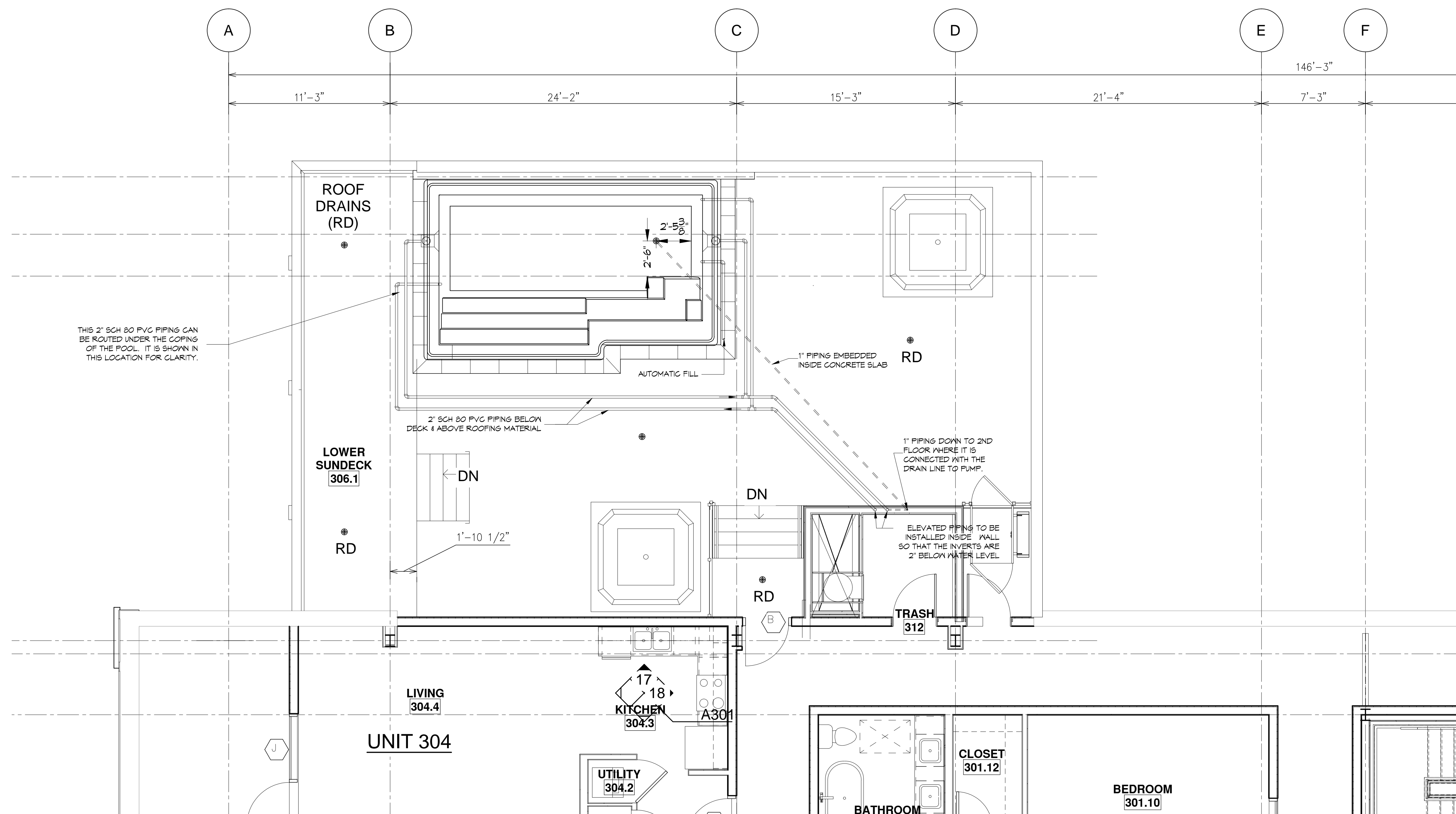
1 3rd FLOOR POOL PIPING PLAN SCALE: 1/4" = 1'-0"
