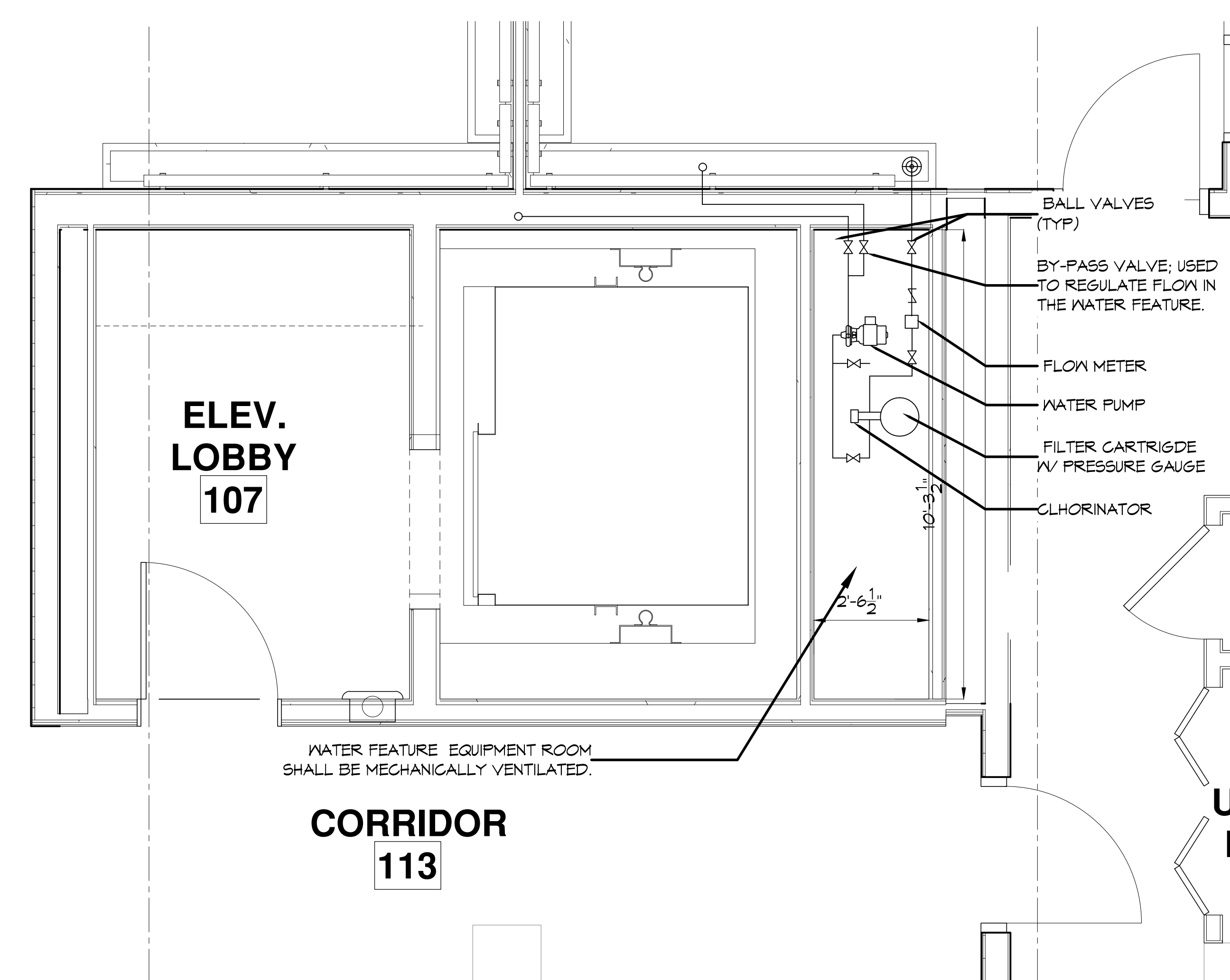
2 POOL EQUIP ROOM SCALE: 1/4" = 1'-0" 2 WATER FALL & EQUIPMENT ROOM SCALE: 1/2" = 1'-0"
