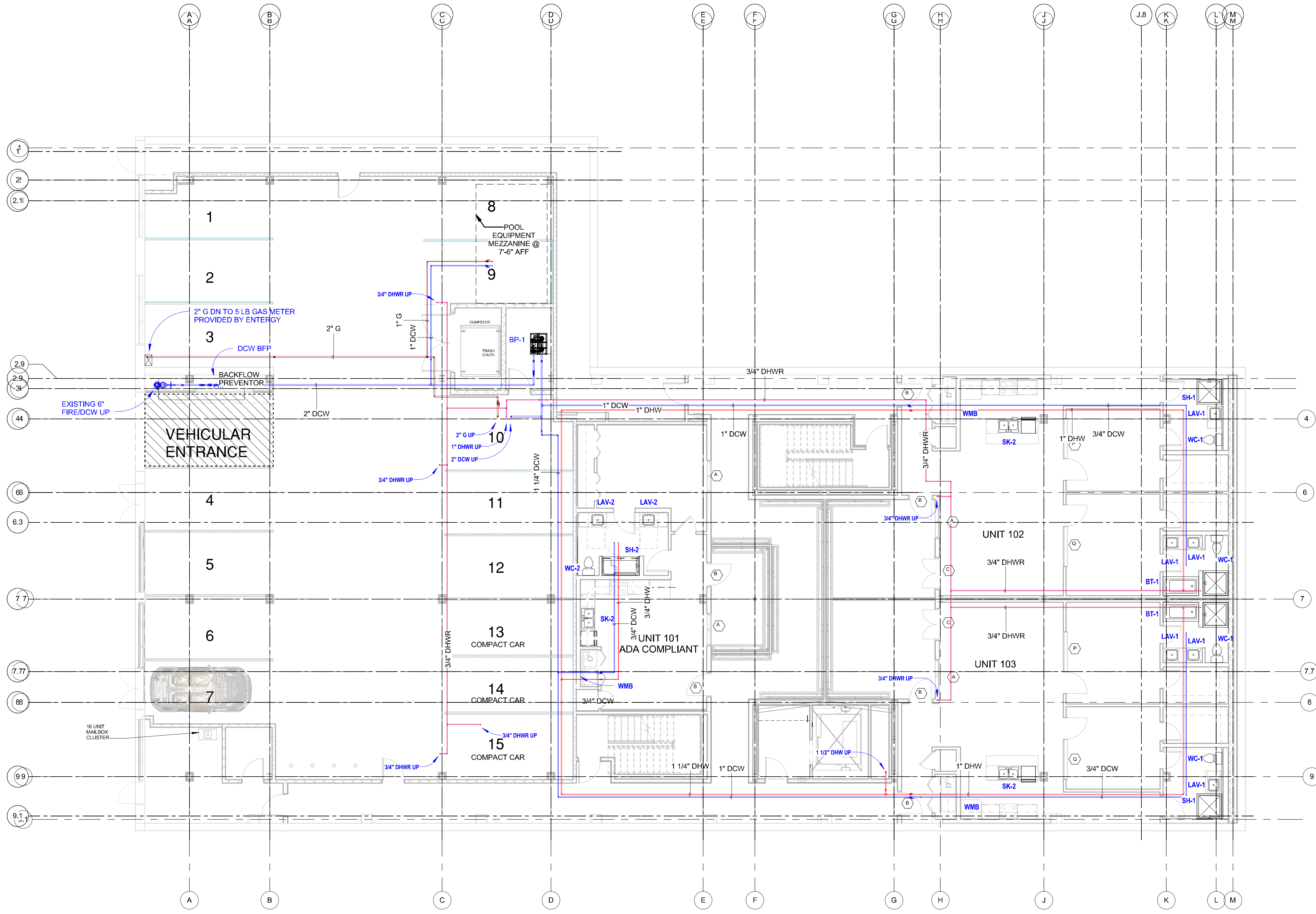
1 1st FLOOR - PLUMBING - WATER 1/8" = 1'-0"
