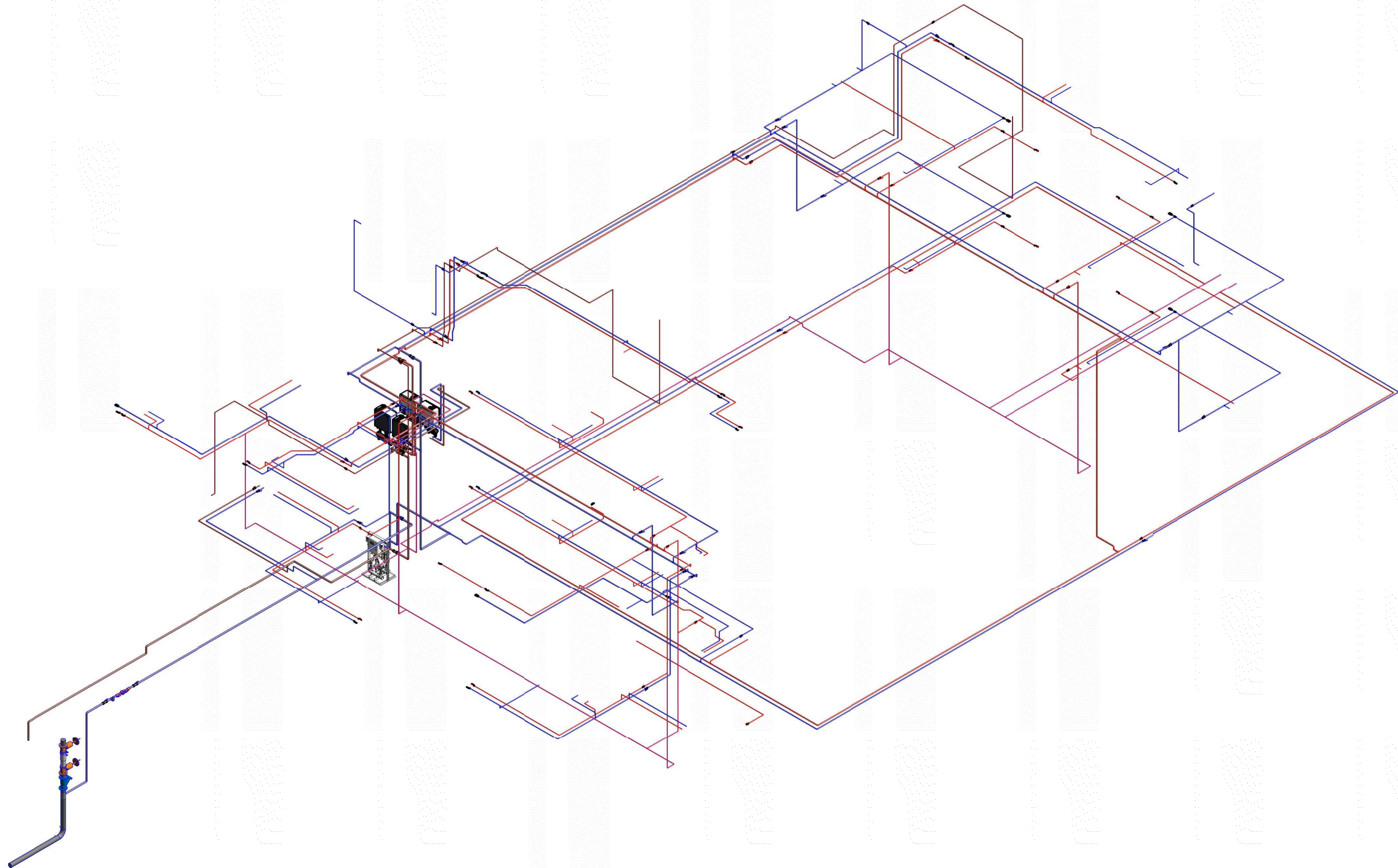
1 WATER ISOMETRIC
