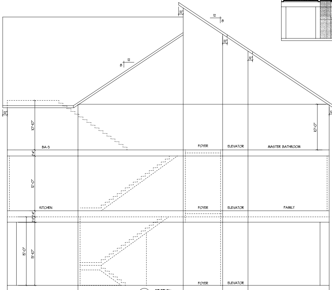
SECTION SCALE 1/4" = 1'-0"
