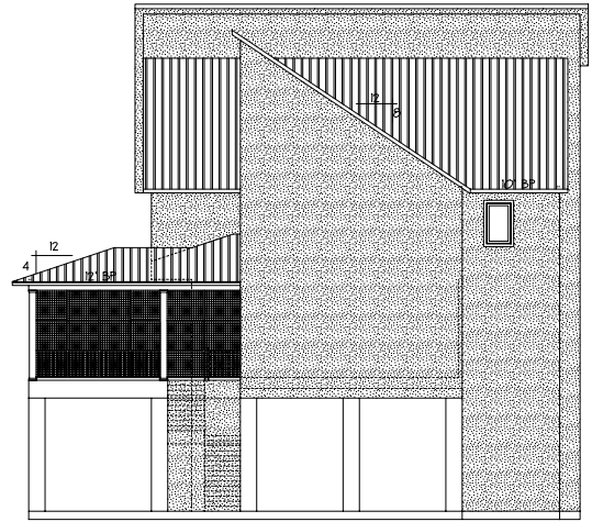
LEFT SIDE ELEVATION SCALE 1/8" = 1'-0"
