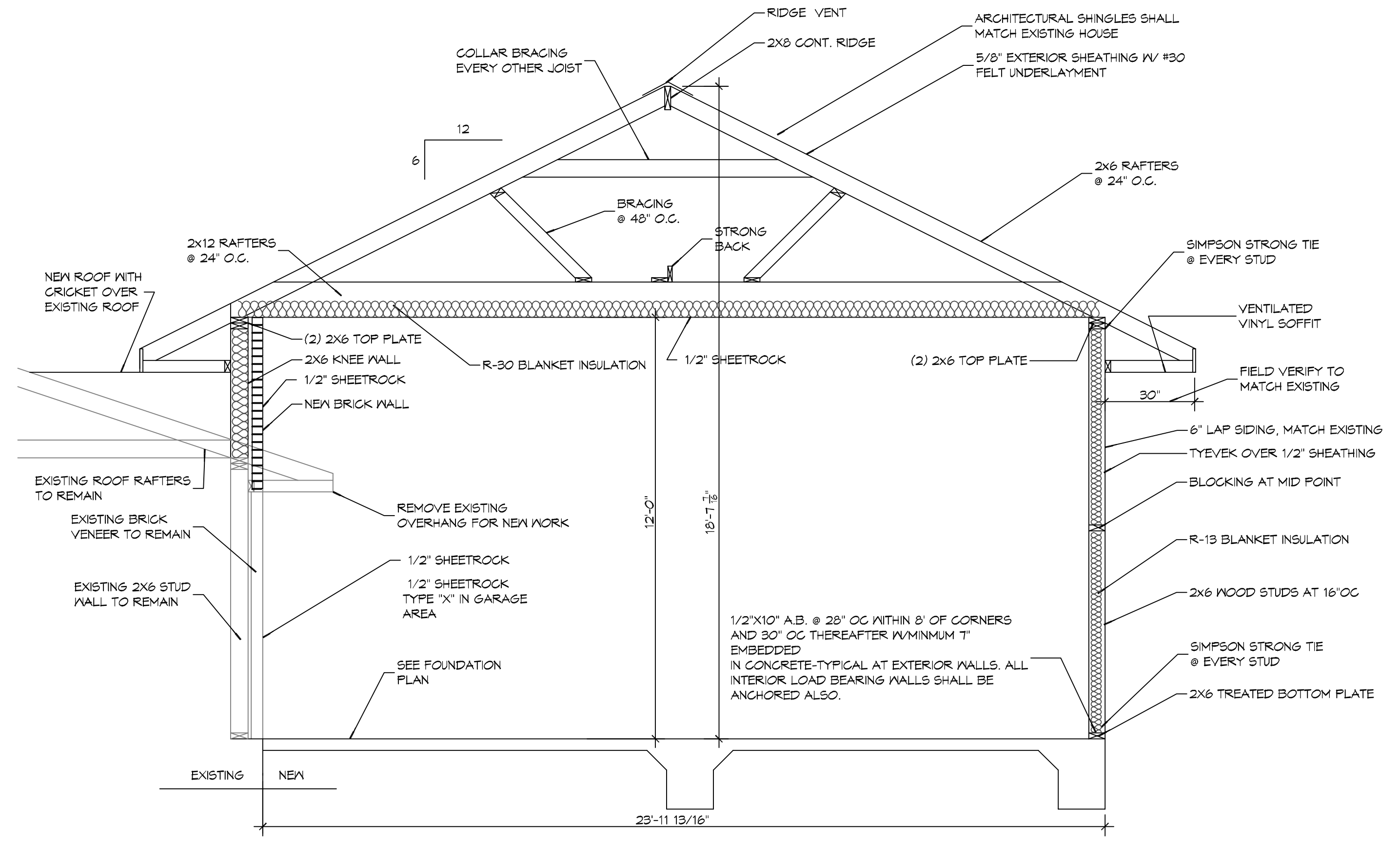
TYPICAL SECTION
