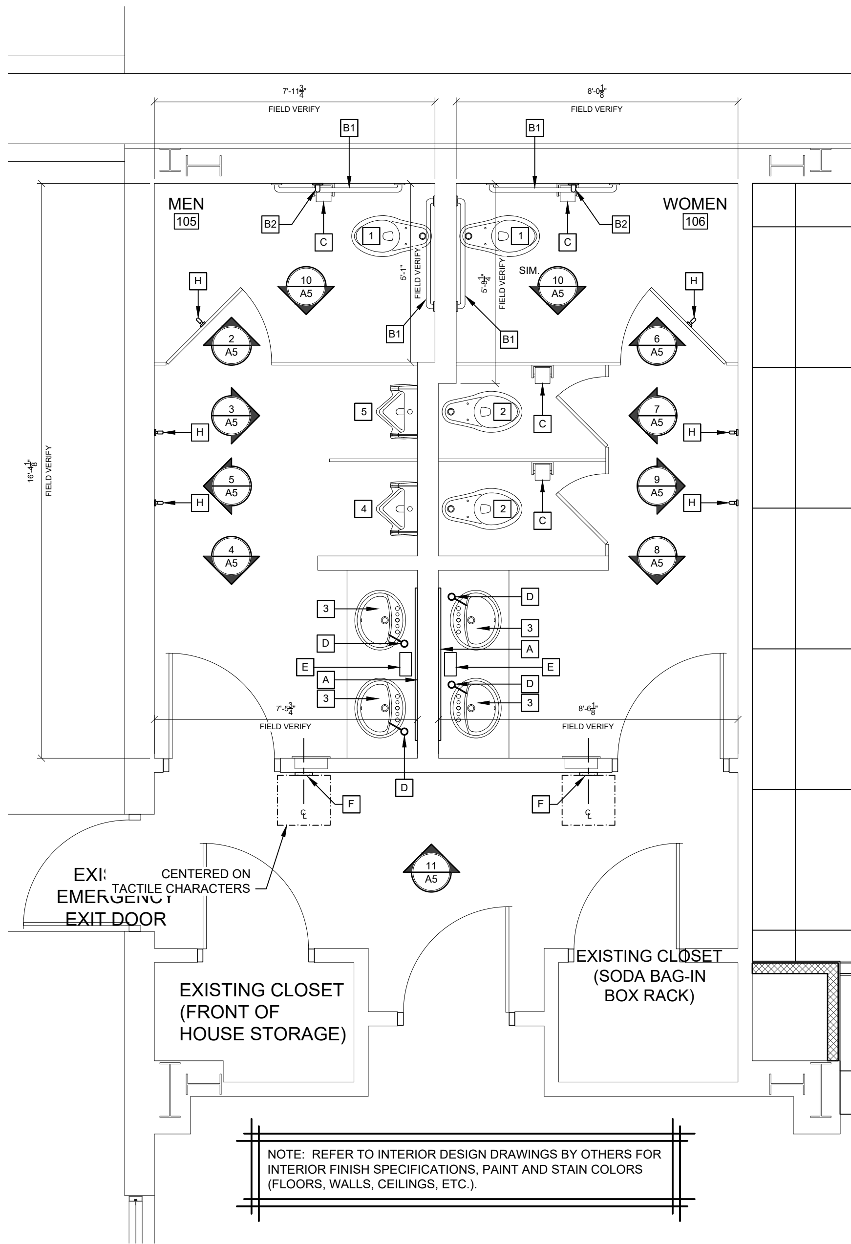
1 ENLARGED RESTROOM PLAN SCALE: 3/8" = 1'-0"
