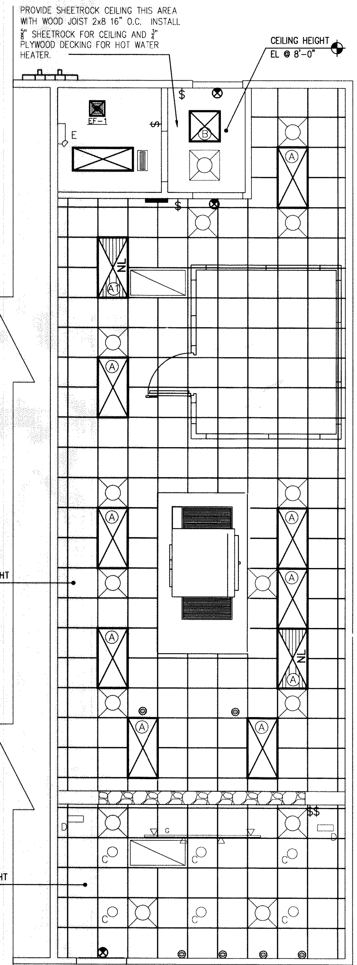
REFLECTED CEILING PLAN SCALE: 1/4" = 1'-0"
