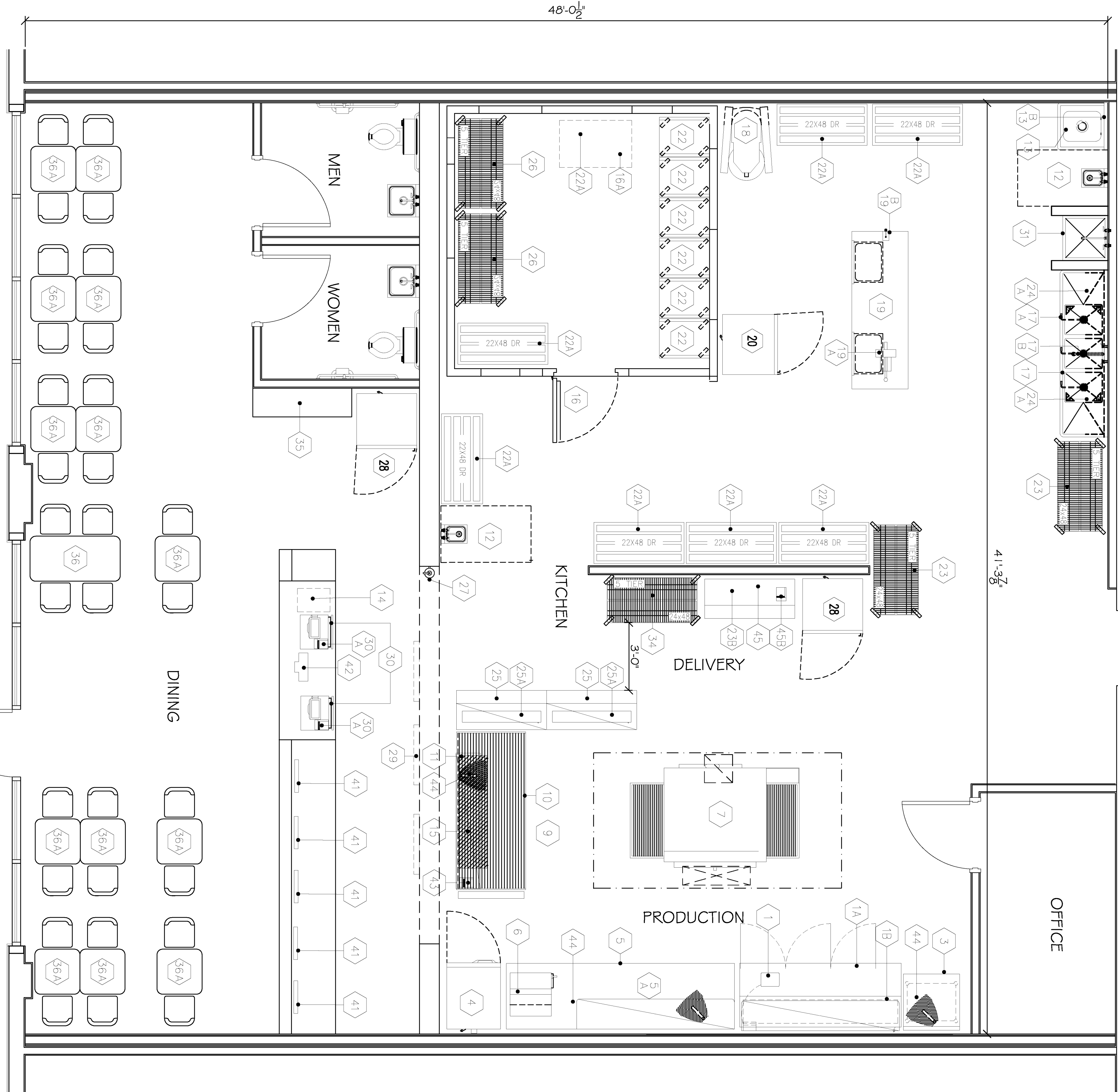
EQUIPMENT PLAN SCALE: 3/8" = 1'-0"
