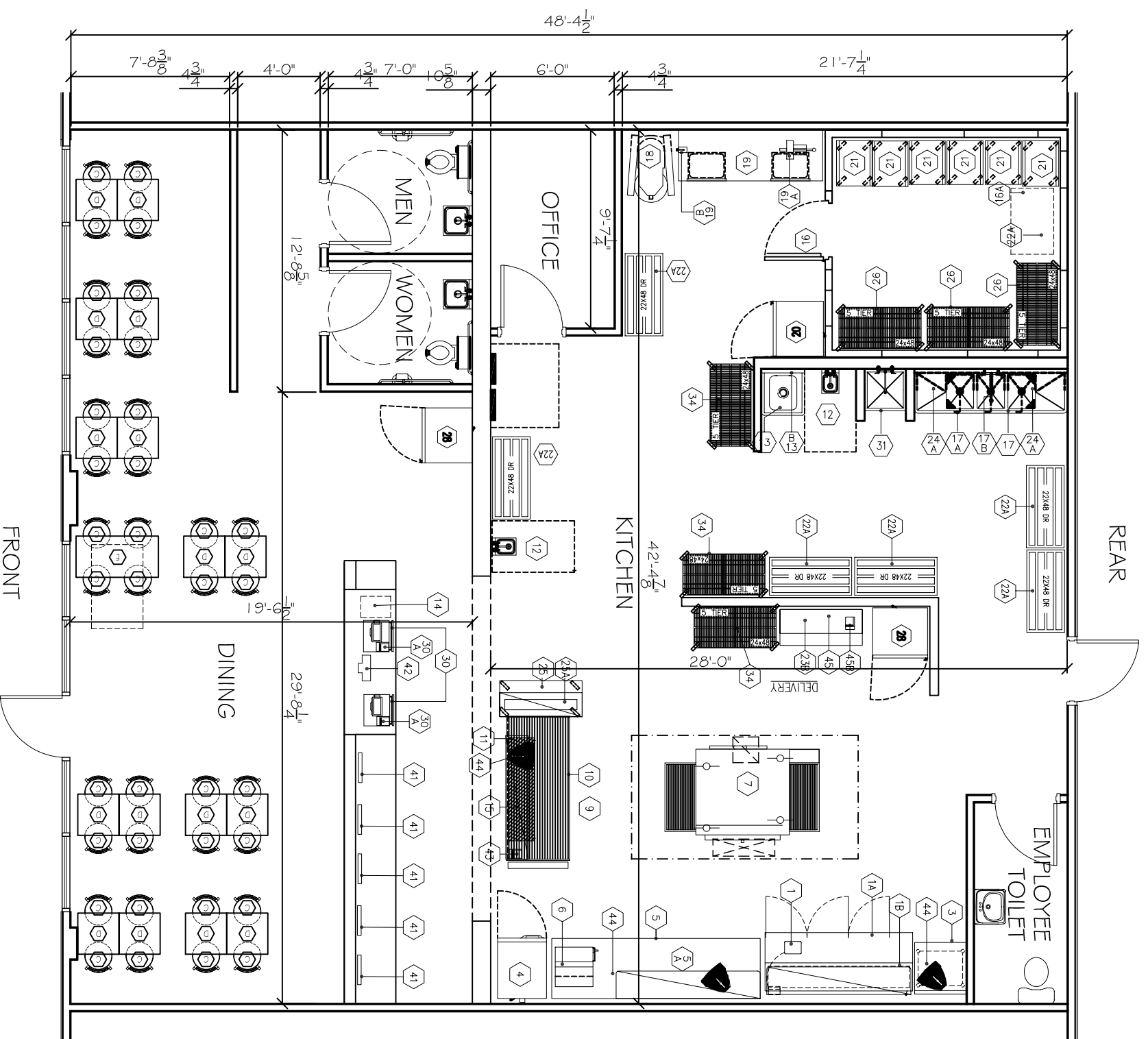
FLOOR PLAN OPTION #2 SCALE: 3/8" = 1'-0"
