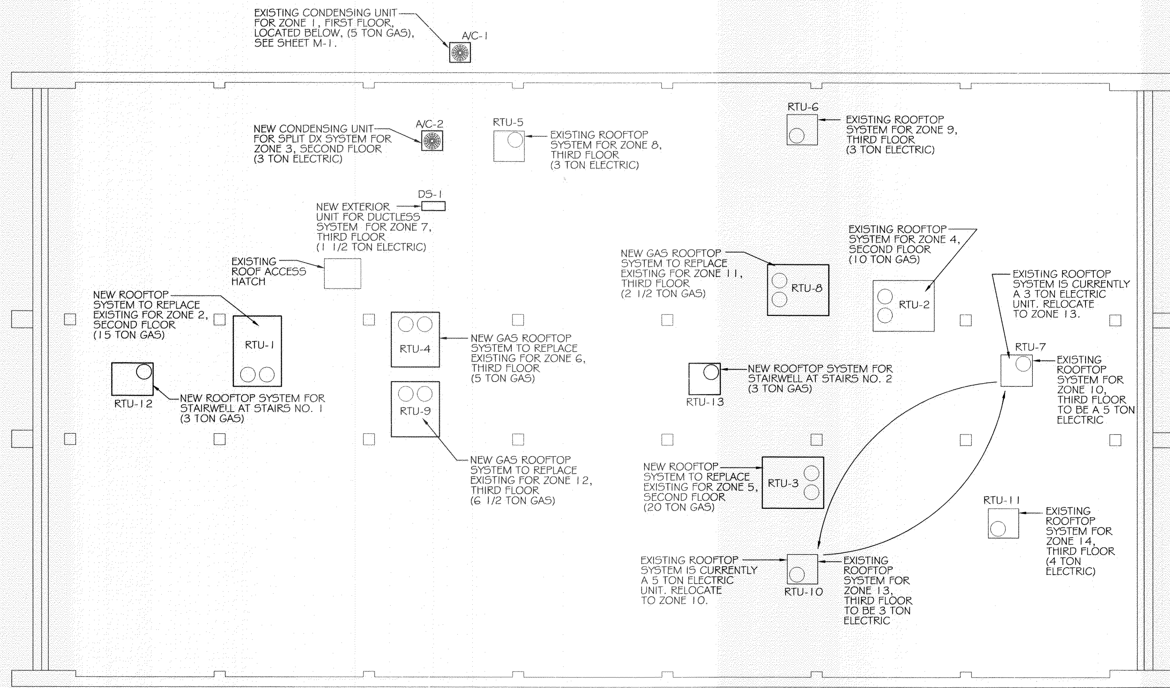
ROOF MECHANICAL EQUIPMENT PLAN SCALE: 1/8"=1'
