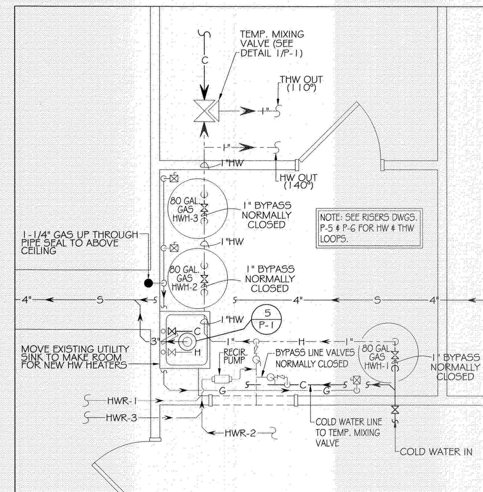
WATER HEATER ROOM LAYOUT PLAN
